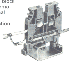
Figure 1. MTC 6 with Shield Connector
