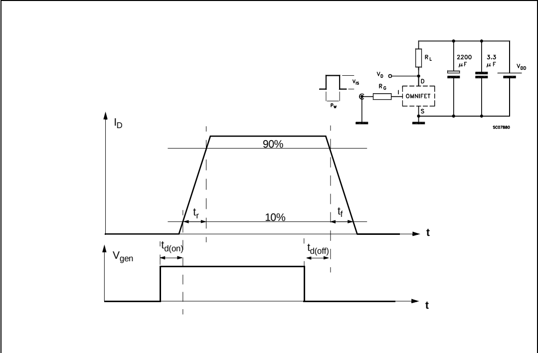
Figure 4. Switching time test circuit for resistive load
