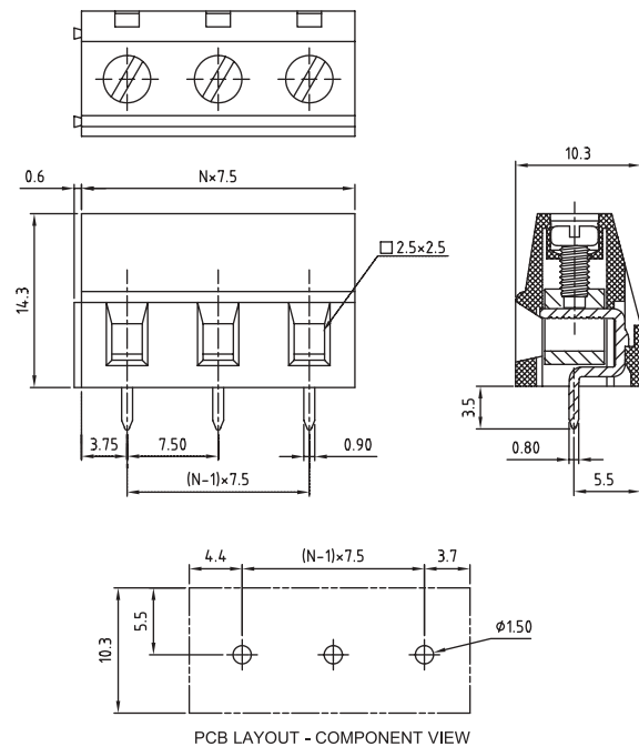
PCB LAYOUT - COMPONENT VIEW
