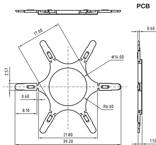
PCB
