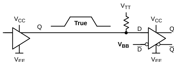
Figure 4. Standard SE Receivers with V_{BB}
