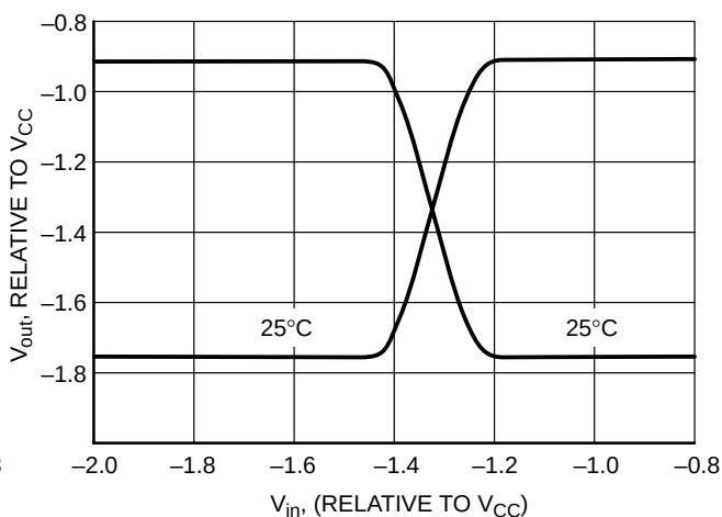
Figure 14. 100E Series V_{in} vs. V_{out} Transfer Curves
