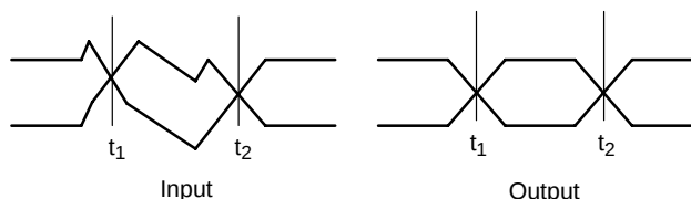
Figure 10. Differential Input High Noise Immunity
