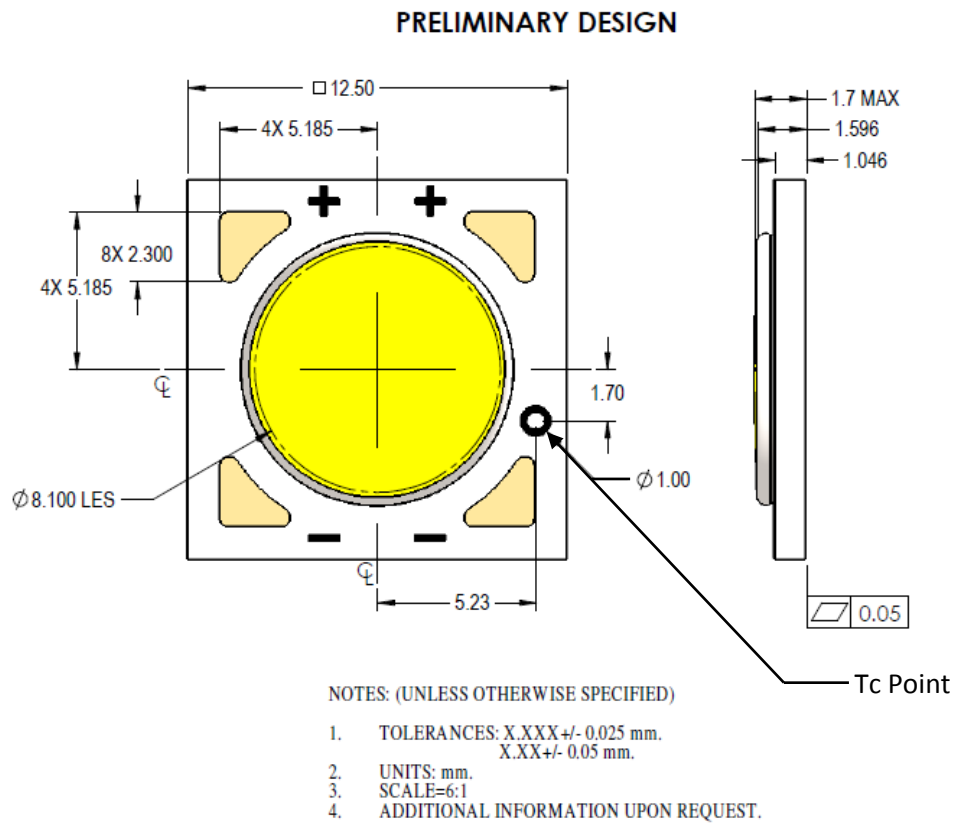
Figure 12: Drawing for V8 Arrays
