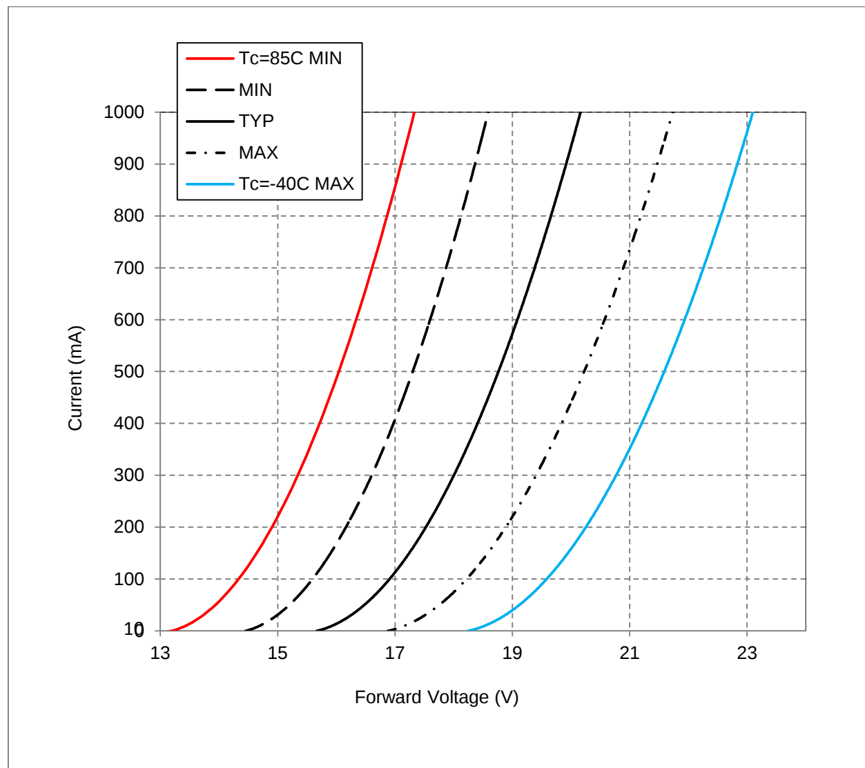
Figure 3: Typical Current vs. Voltage – BXRE-xxx0800-B-xx
