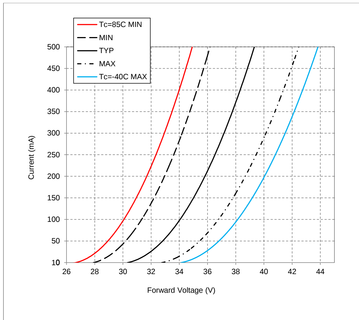
Figure 2: Typical Current vs. Voltage – BXRE-xxx0800-A-xx
