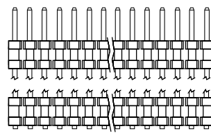
SURFACE MOUNT
