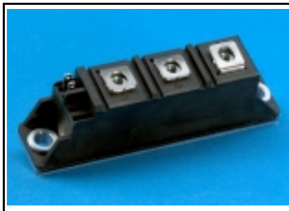
CD42_90A, CD47_90A Dual SCR/Diode Isolated POW-R-BLOK™ Module 90 Amperes / Up to 1600 Volts
