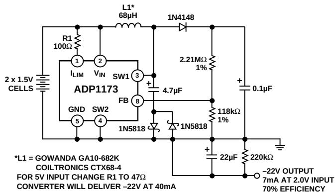
Figure 24. 3 V–22 V LCD Bias Generator
