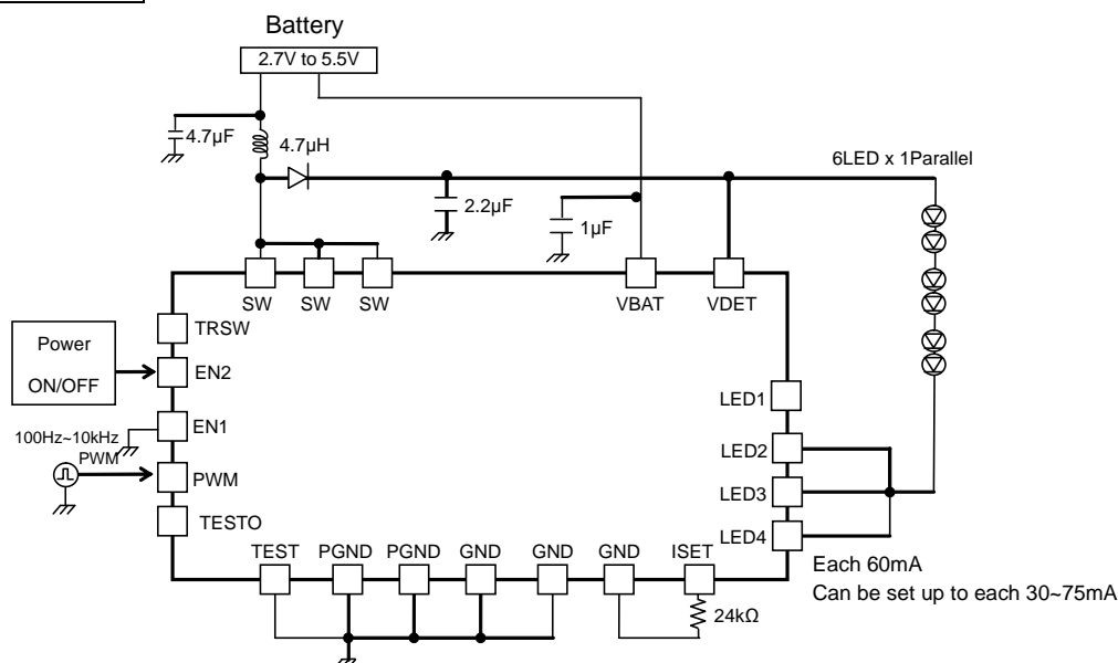
Figure 22. 6 series×1 parallel, LED current 60mA setting Current driver PWM application
