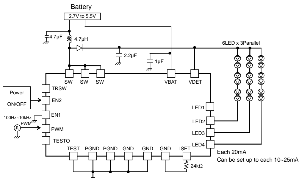
Figure 15. 6 seriesx3 parallel, LED current 20mA setting Current driver PWM application
