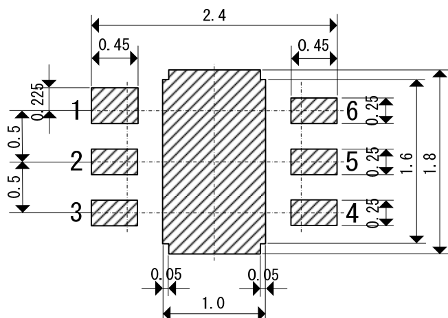
● USP-6C Reference Pattern Layout (unit: mm)
