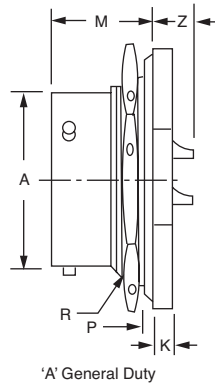
'A' General Duty
