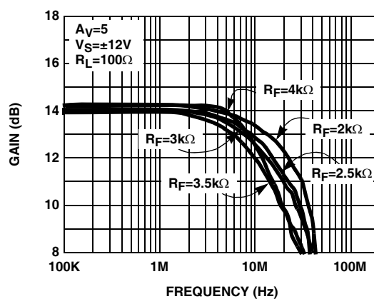
FIGURE 6. DIFFERENTIAL FREQUENCY RESPONSE vs R_F (FULL POWER MODE)
