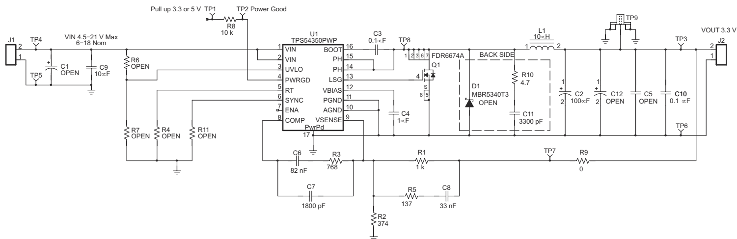
Figure 4-1. TPS54350EVM-235 Schematic
