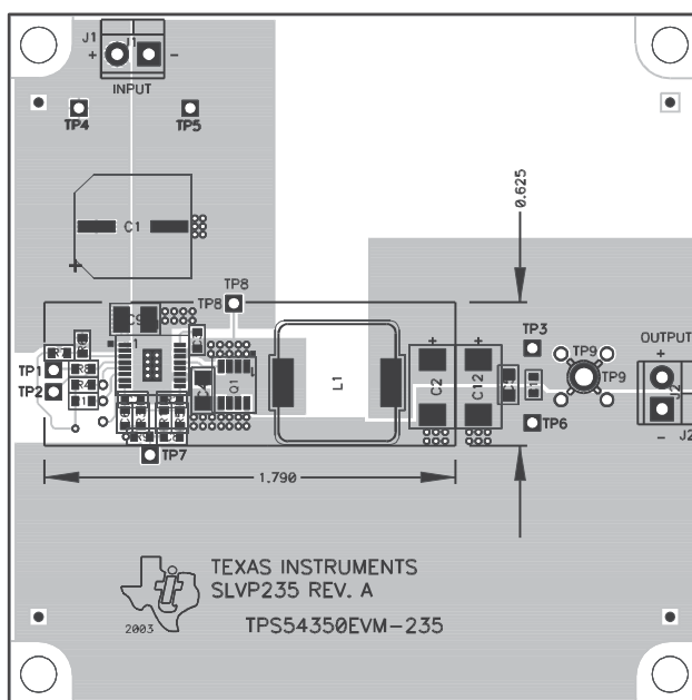
Figure 3-3. Top Side Assmebly
