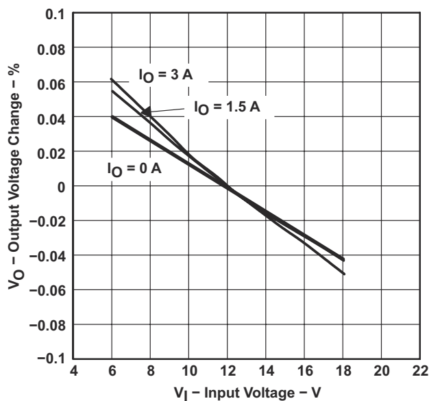
Figure 2-5. Line Regulation
