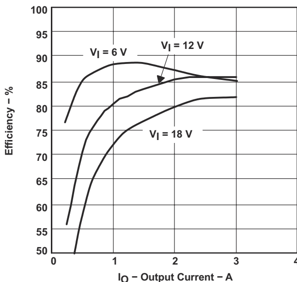
Figure 2-2. Measured Efficiency
