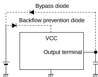
Fig.27 Bypass Diode
