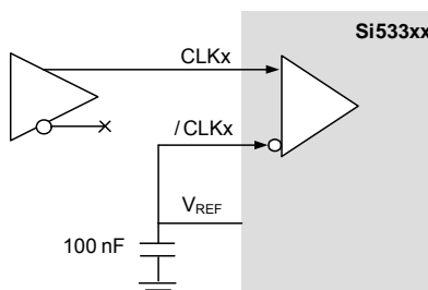
Figure 6. Using Voltage Reference with Single-Ended Input Clock
