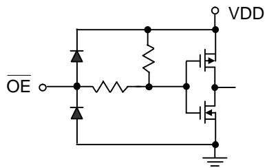
\overline{\text{OE}} (CA2) terminal
