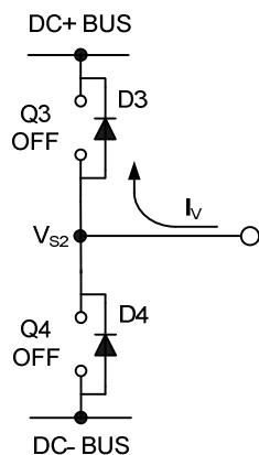
Figure 28: D3 conducting
