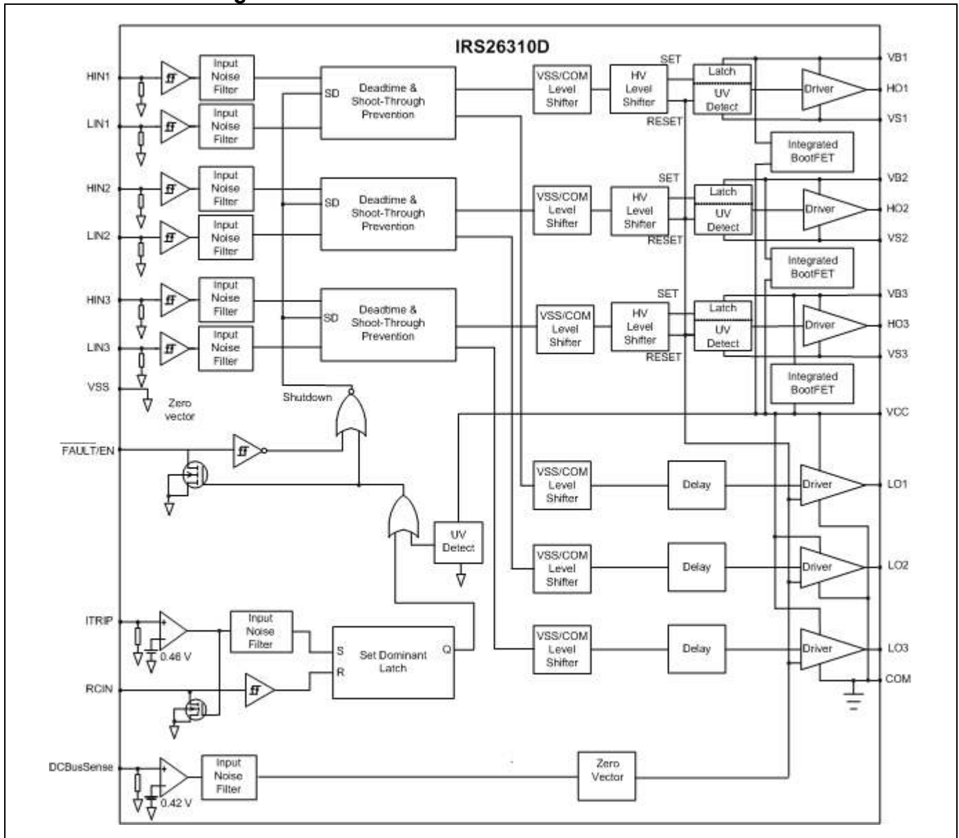
Functional Block Diagram: IRS26310DJ
