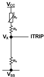
Figure 14: Programming over-temperature protection
