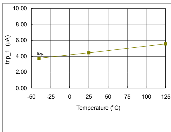
Figure 60: I_{TRIP+} vs. temperature
