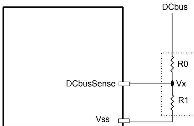
Figure 16: Programming the DC bus over-voltage protection
