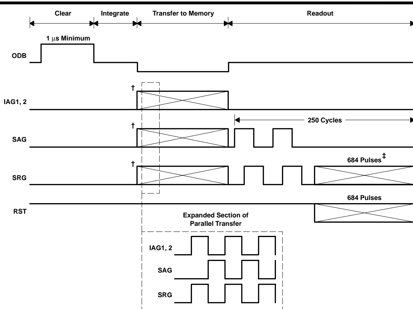
Figure 3. Interlace Timing
