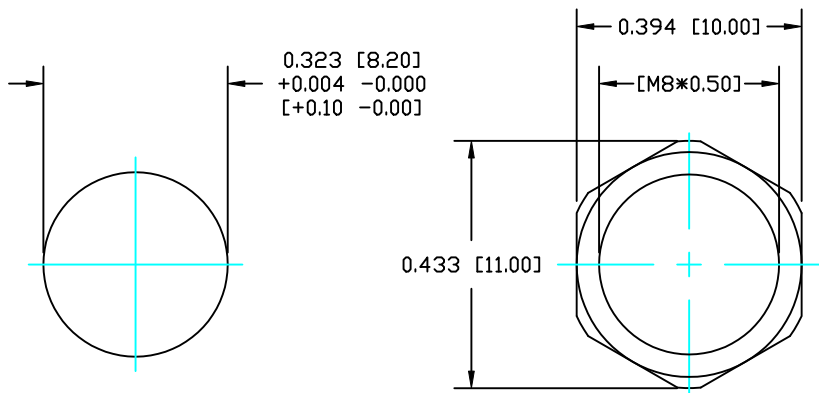
PANEL CUTOUT
