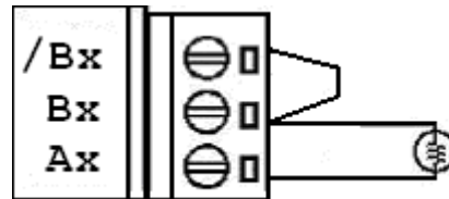
2-wire RTD connection
