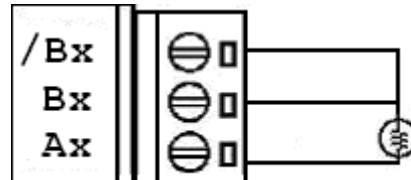
3-wire RTD connection
