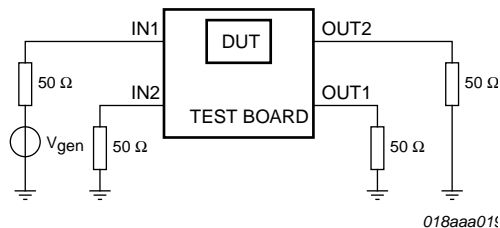
Fig 5. Crosstalk measurement configuration
