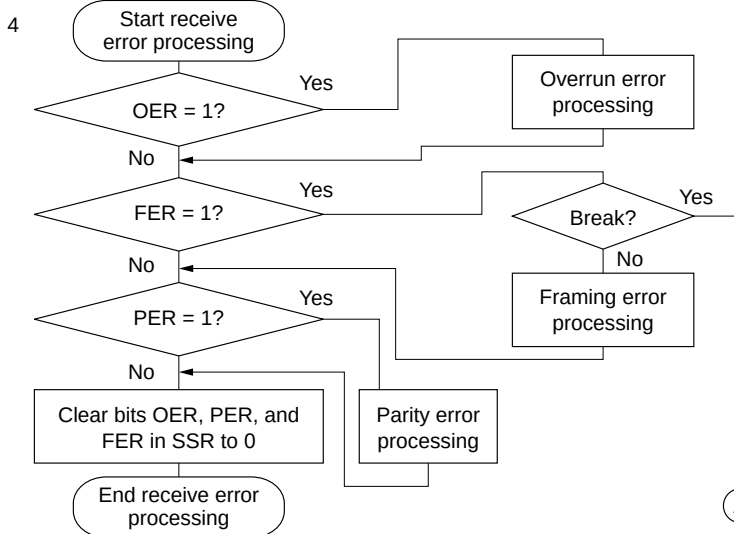
Figure 10.14 Typical Serial Data Receiving Flow Chart in Asynchronous Mode
