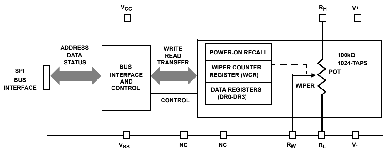
FIGURE 1. FUNCTIONAL DIAGRAM
