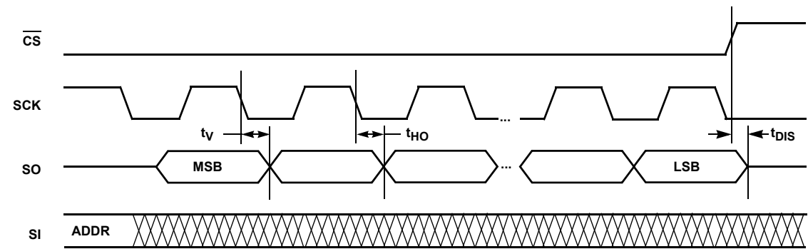
FIGURE 8. OUTPUT TIMING
