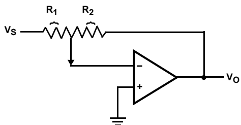
FIGURE 20. INVERTING AMPLIFIER
