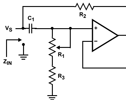
FIGURE 21. EQUIVALENT L-R CIRCUIT
