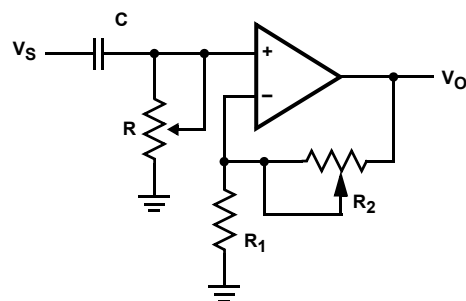
FIGURE 19. FILTER
