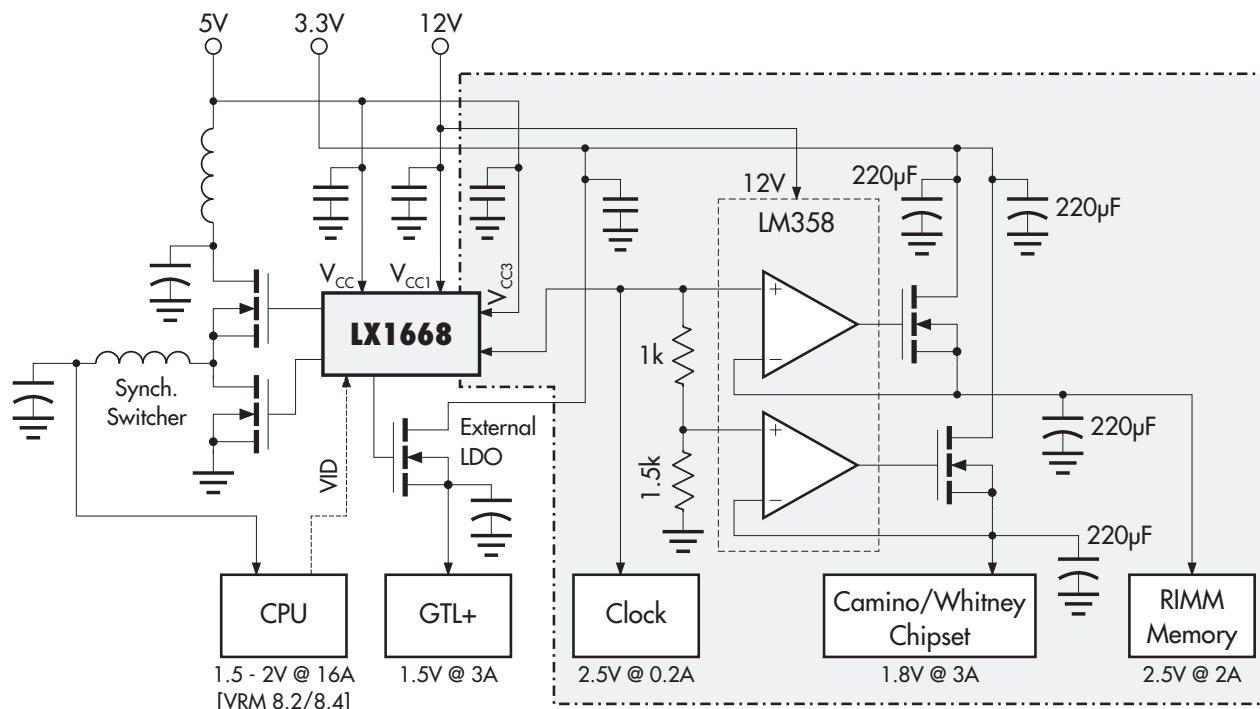
FIGURE 6 — Pentium III Processor Power Supply (Whitney / Camino Chipsets)
