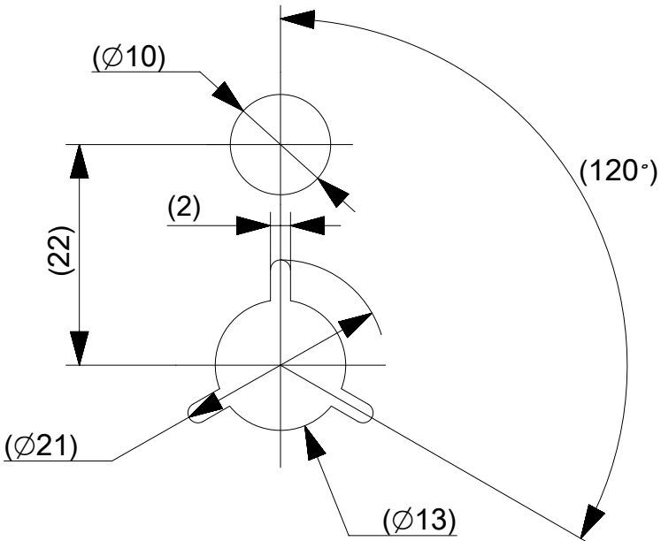
DETAIL "Z"
