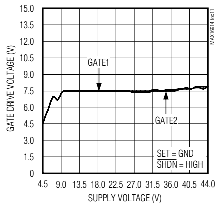
V_{CC} - V_{GATE} vs. INPUT VOLTAGE
