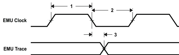
Figure 7-67. Trace Timing
