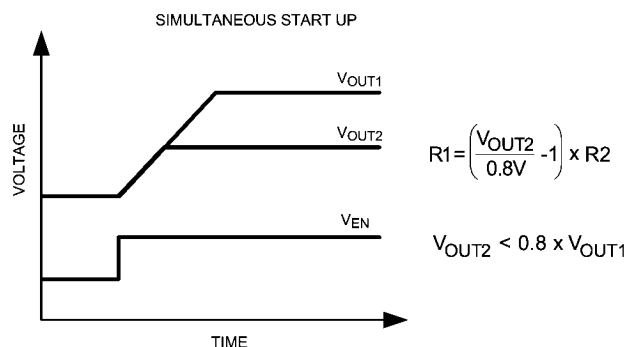
FIGURE 6. Sequencing LM20124 with Precision Enable
