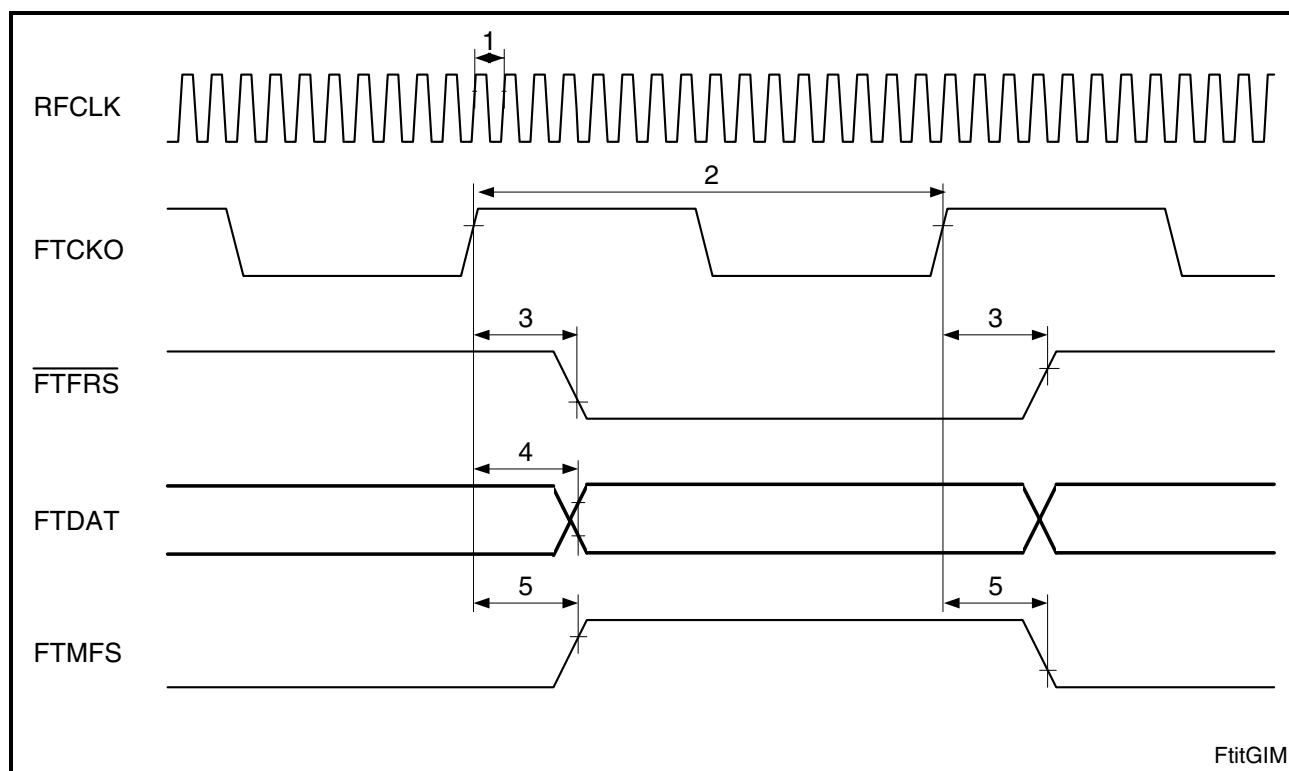
Figure 60 Framing Transmit Interface Timing in GIM
