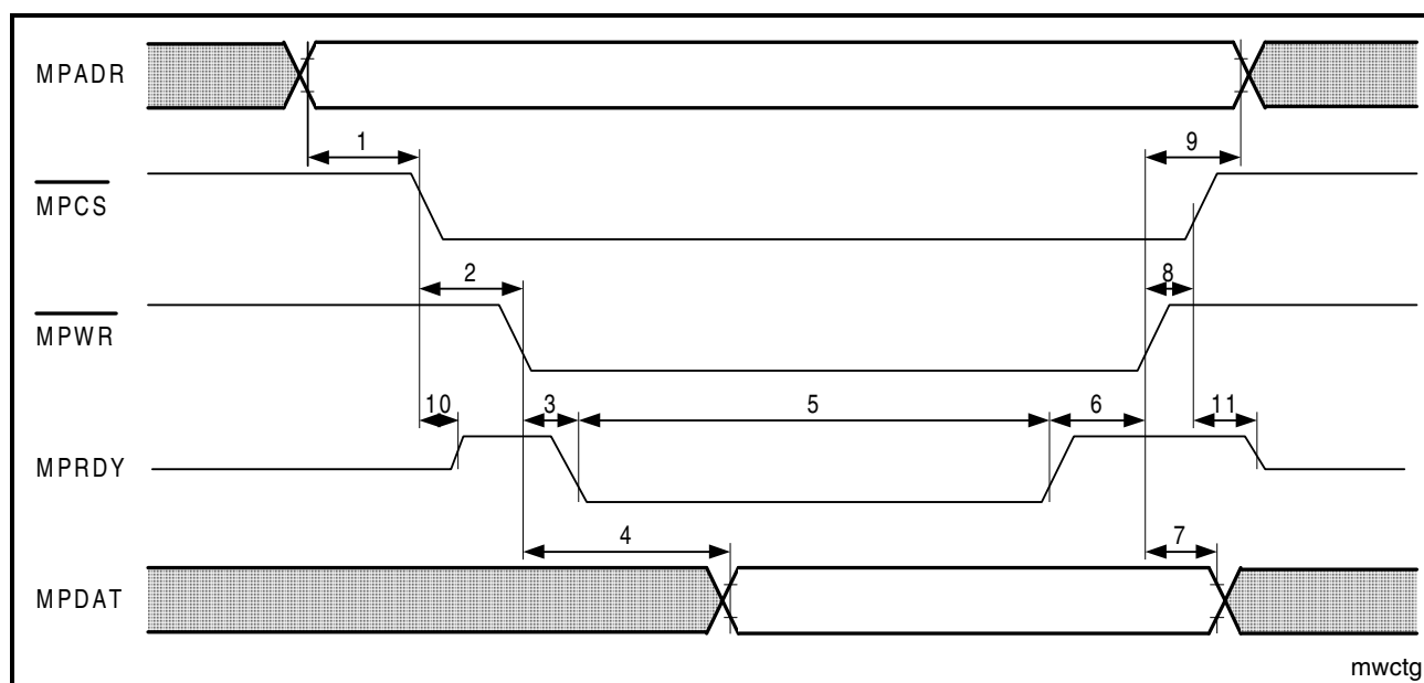
Figure 68 Intel Mode Write Cycle Timing Diagram
