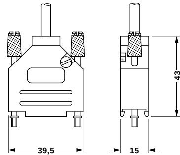
SCT-D-SUB 15 KG
