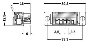
SCT-D-SUB 15 KG
