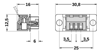
SCT-D-SUB 9-KG
