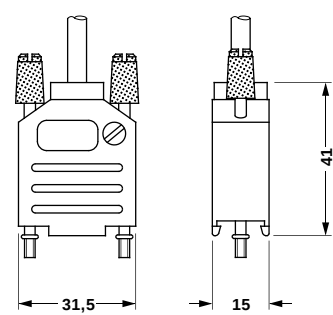
SCT-D-SUB 9-KG
