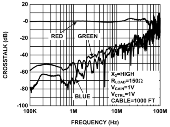
FIGURE 20. RED CROSSTALK
