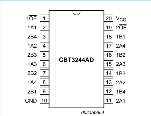
Fig 3. Pin configuration for SO20
