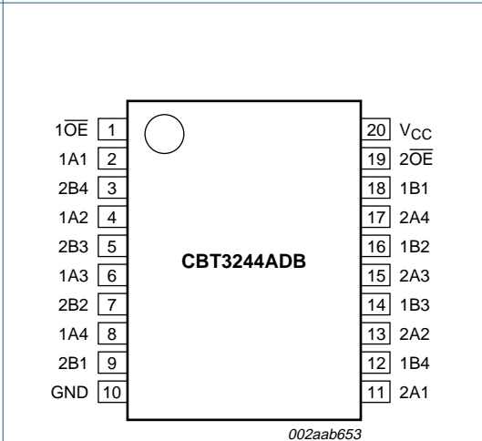
Fig 5. Pin configuration for SSOP20
