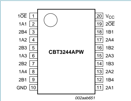
Fig 2. Pin configuration for TSSOP20
