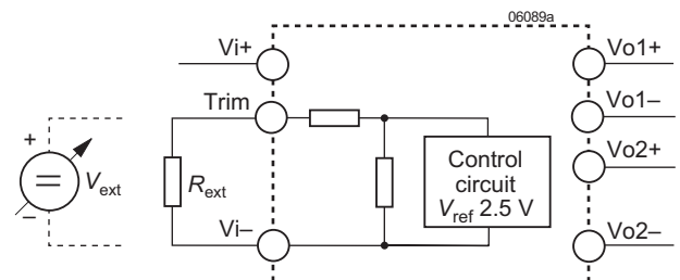
Fig. 16 Output voltage control for double-output models (without option R) by means of the Trim input.
