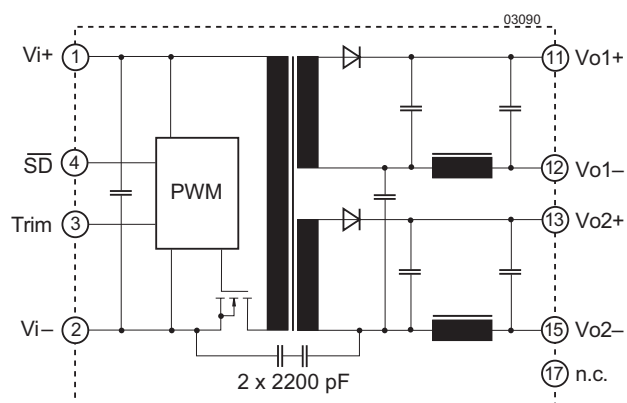
Fig. 3 Block diagram of double-output models
