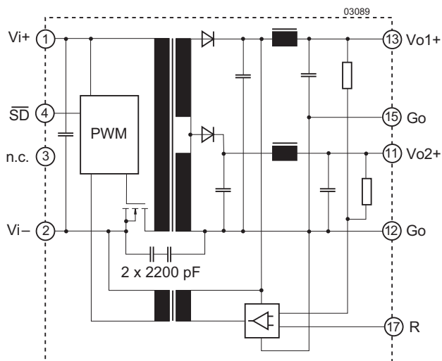
Fig. 2 Block diagram of -0503-models
