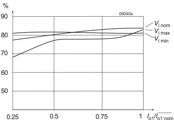
Fig. 12c Efficiency versus input voltage and load. Typical values (48IMS15-12-12-9)
