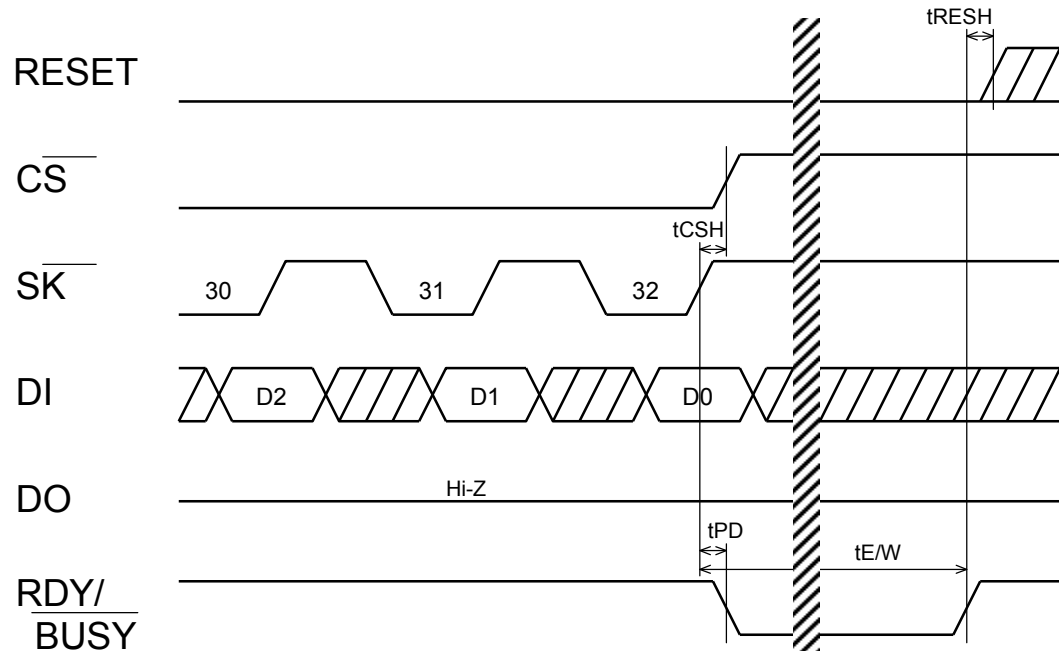
WRITE Ready / Busy Signal Output (RDY/ BUSY pin)
