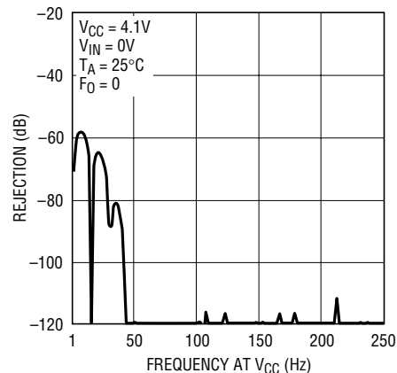
Rejection vs Frequency at V_{\text{CC}}
