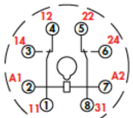
NEMA IEC Wiring Diagram Bottom View
