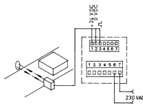
Count pulses from a light barrier
