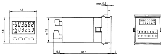
903 panel cut-out 45 x 45 mm
