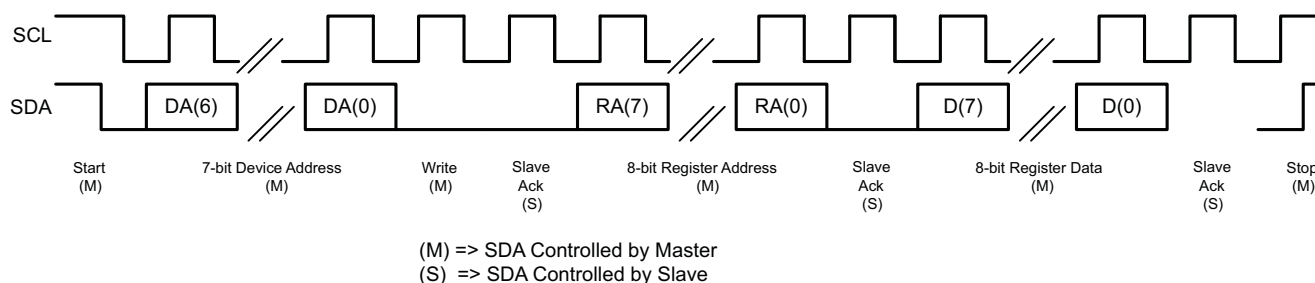
Figure 5-32. I 2 C Write
