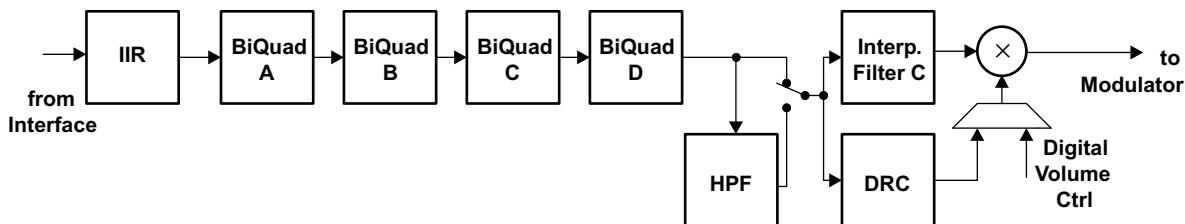
Figure 5-8. Signal Chain for PRB_P21
