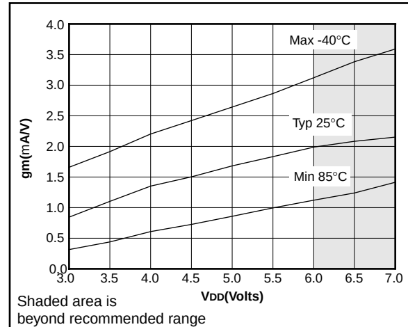
FIGURE 21-20: TRANSCONDUCTANCE(gm) OF LP OSCILLATOR vs. V_{DD}
