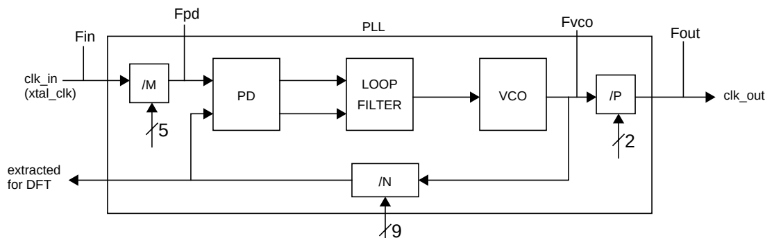
Figure 2: PLL Block Diagram
