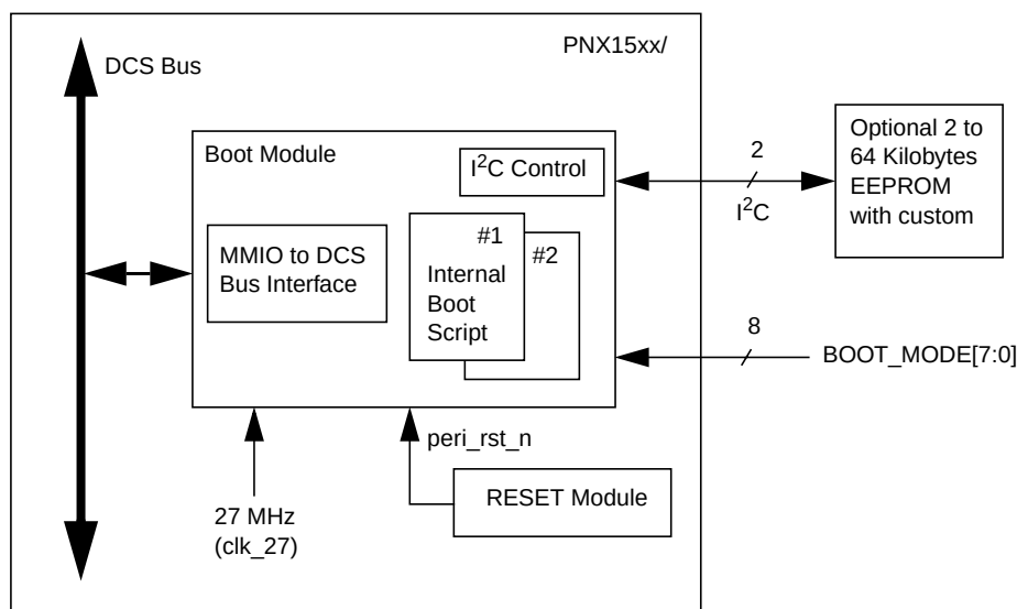
Figure 1: Boot Block Diagram
