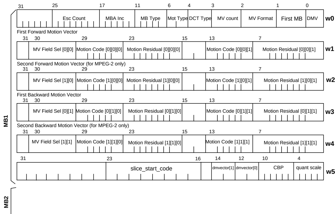
Figure 2: MPEG-2 Macro Block Header Output Format
