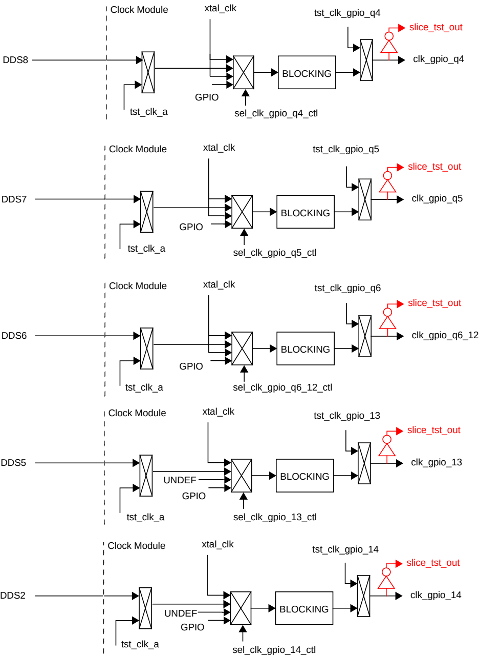
Figure 14: GPIO Clocks
