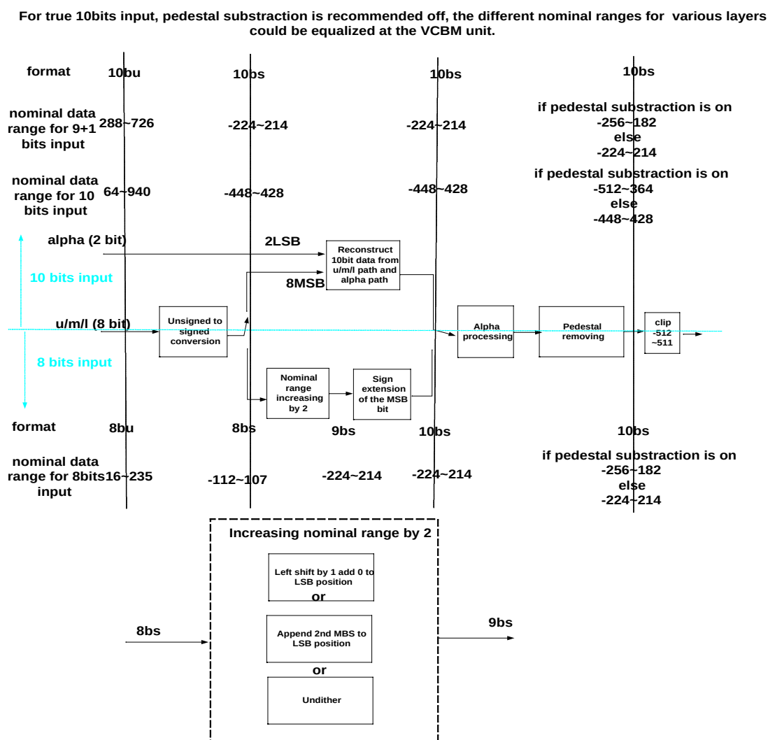
Figure 3: Undithering and Pedestal Manipulation
