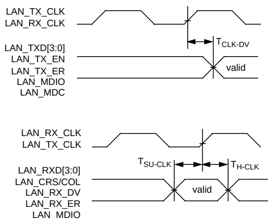
Figure 14: LAN 10/100 I/O Timing in MII Mode
