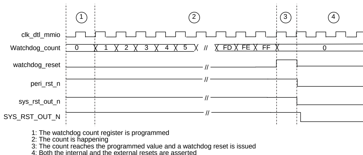
Figure 2: Watchdog in Non Interrupt Mode
