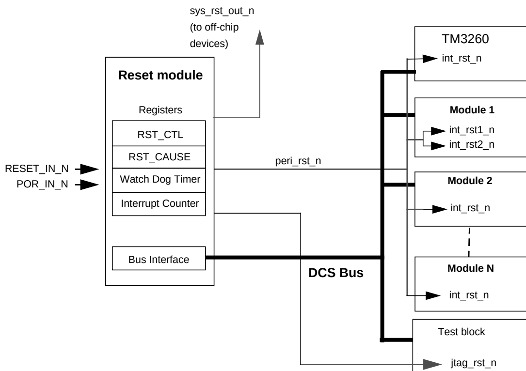
Figure 1: Reset Module Block Diagram
