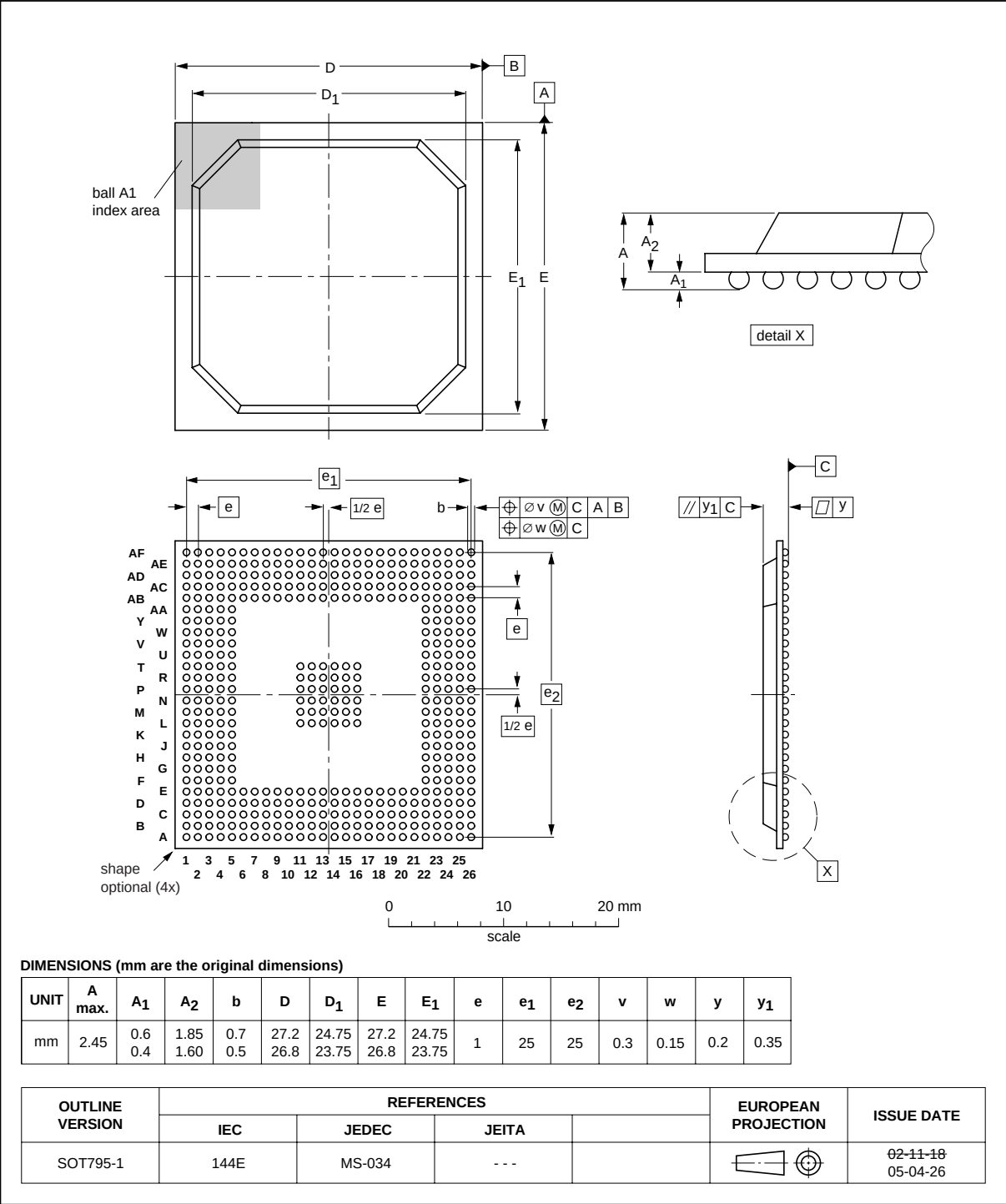
BGA456: plastic ball grid array package; 456 balls; body 27 x 27 x 1.75 mm SOT795-1
