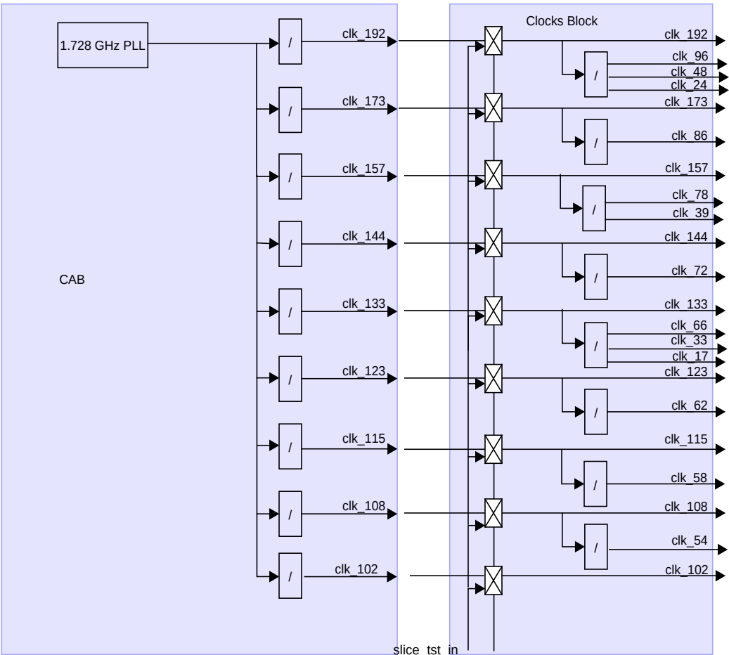
Figure 10: Clock Dividers
