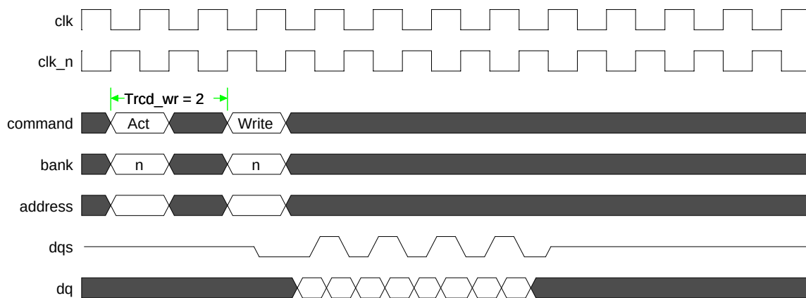
Figure 16: Trcd_wr Timing Parameter
