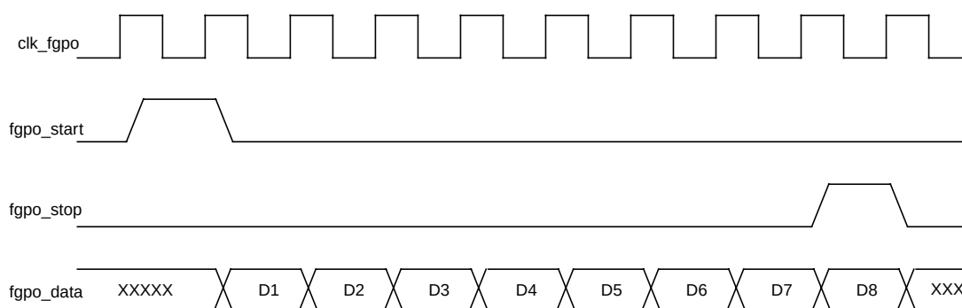
Figure 6: Back-to-back Message Passing Example
