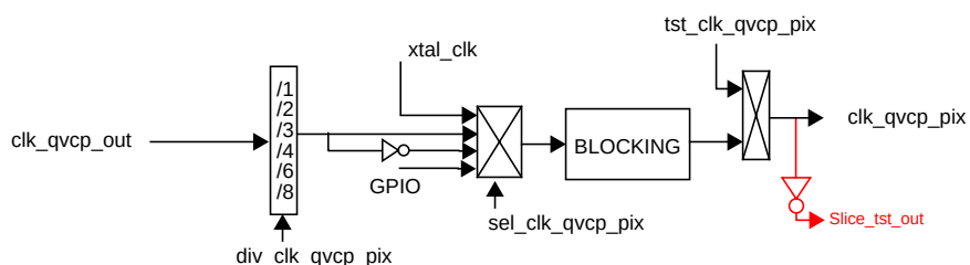
Figure 9: QVCP_PIX Clock
