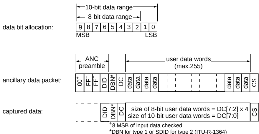
Figure 13: ANC Data Structure
