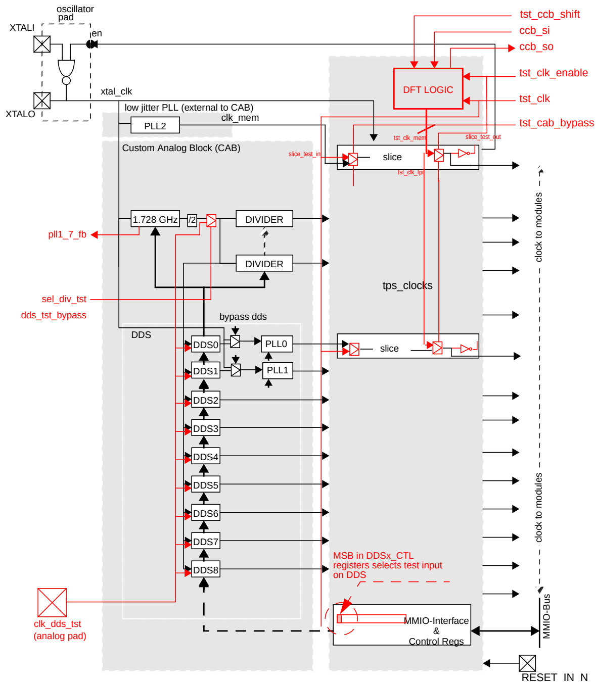
Figure 1: Clock Module Block Diagram
