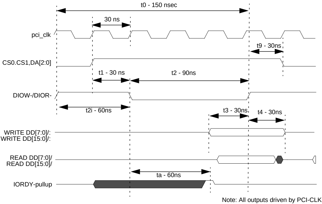
Figure 14: Timings on IDE Bus
