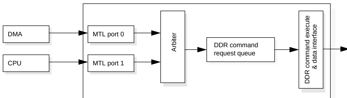
Figure 1: The two MTL Ports of the DDR SDRAM Controller
