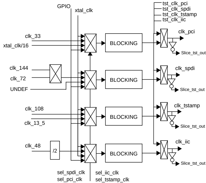
Figure 12: Internal PNX15xx/952x Series Clock from Dividers: PCI, SPDI, LCD and I²C
