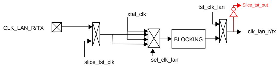
Figure 22: Receive and Transmit LAN Clocks
