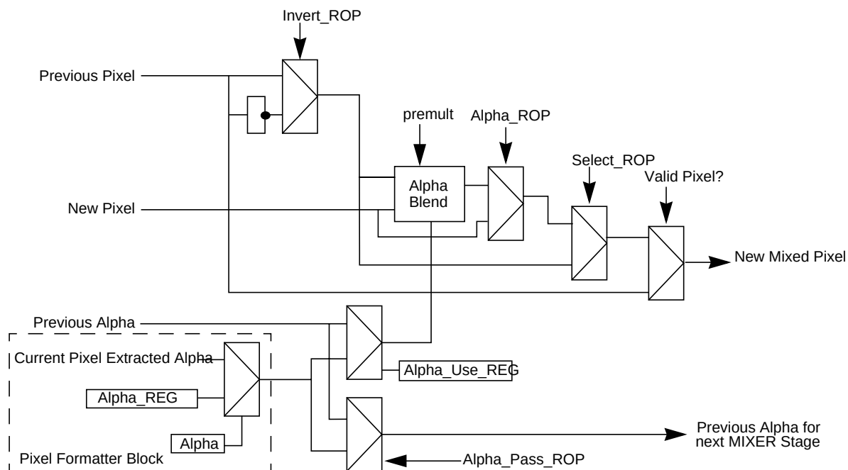
Figure 6: Mixer Block Diagram—Pixel Processing
