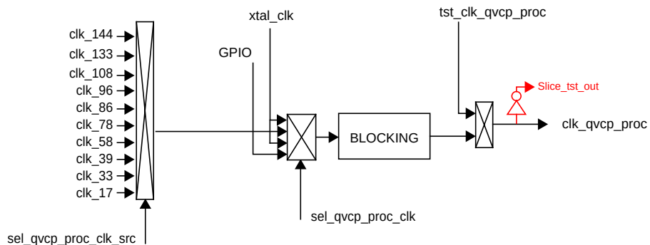
Figure 8: QVCP_PROC Clock
