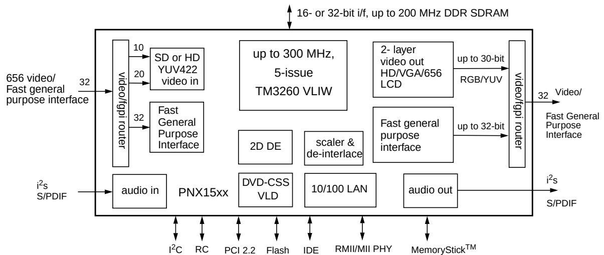
Figure 1: Block Diagram PNX15xx/952x Series
