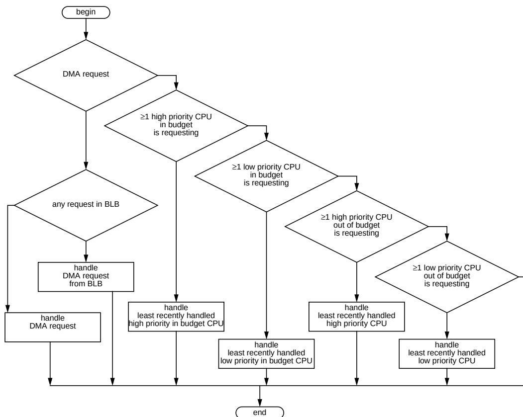
Figure 4: Arbitration when DMA has priority
