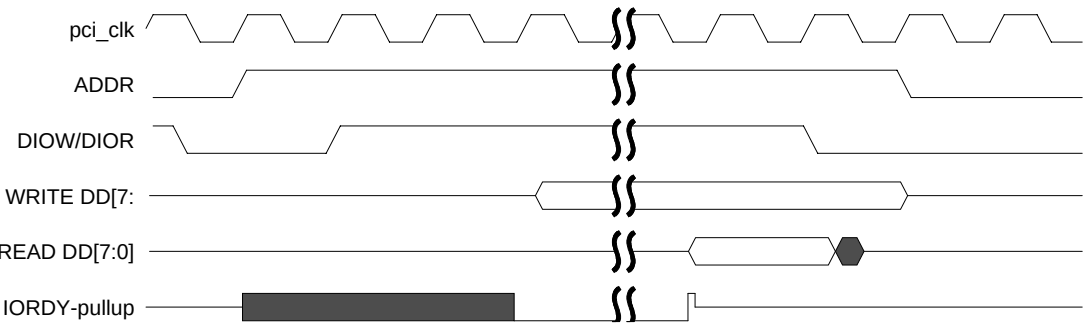
Figure 15: IDE Transaction, Flow Controlled by Device IORDY
