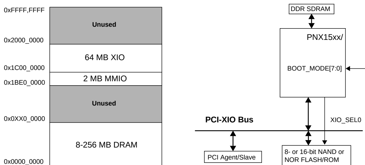
Figure 2: System Memory Map and Block Diagram Configuration for PNX15xx/952x Series in Standalone Mode
