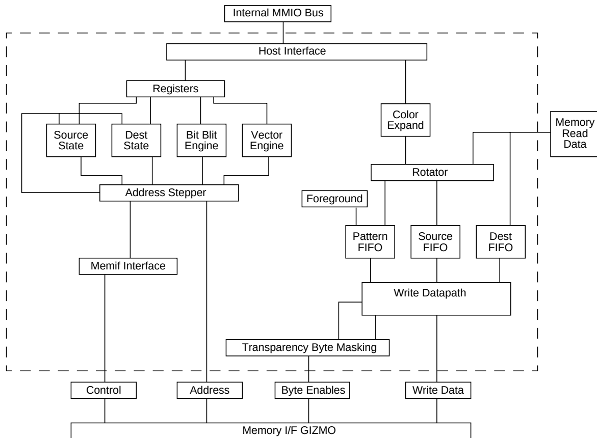
Figure 1: 2D Drawing Engine Block Diagram
