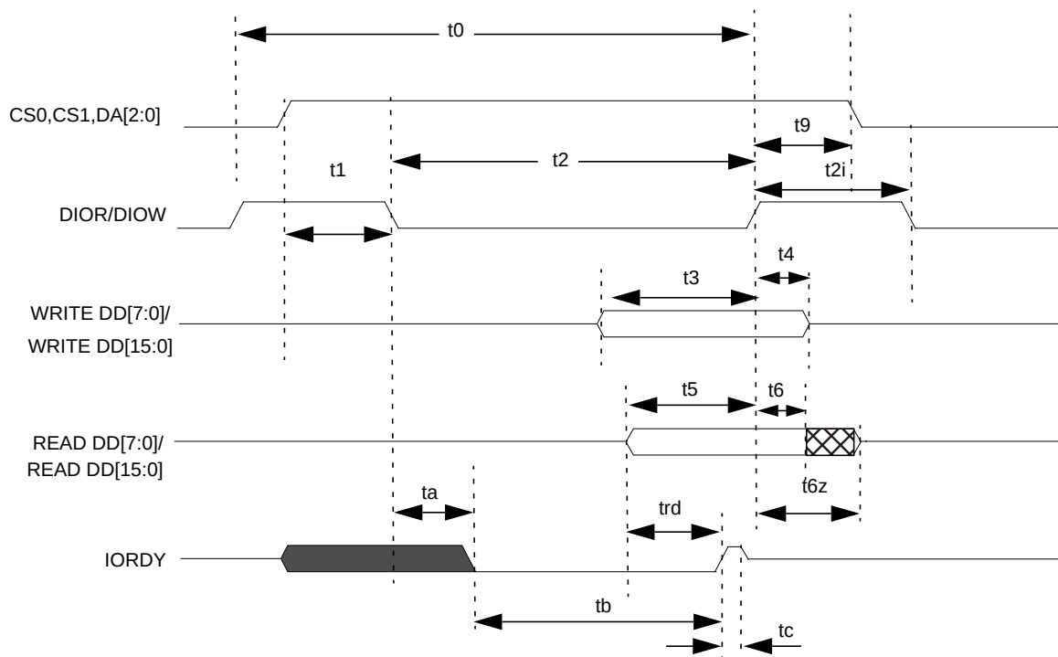
Figure 13: Register Transfer/PIO Data Transfer on IDE
