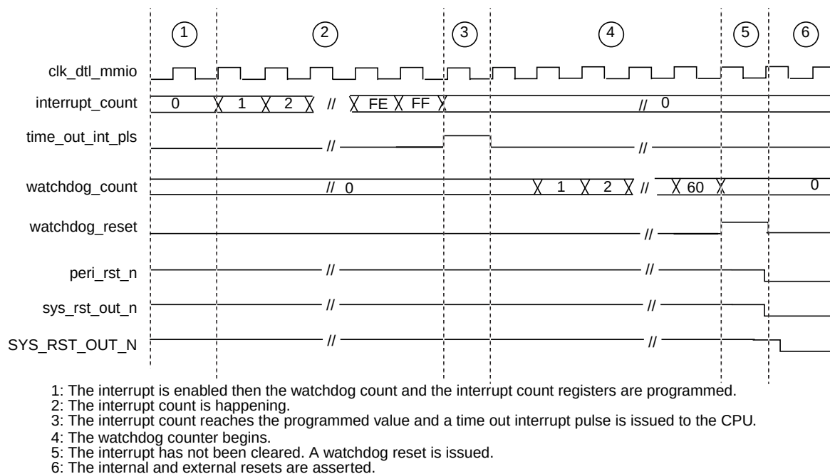
Figure 3: Watchdog in Interrupt Mode
