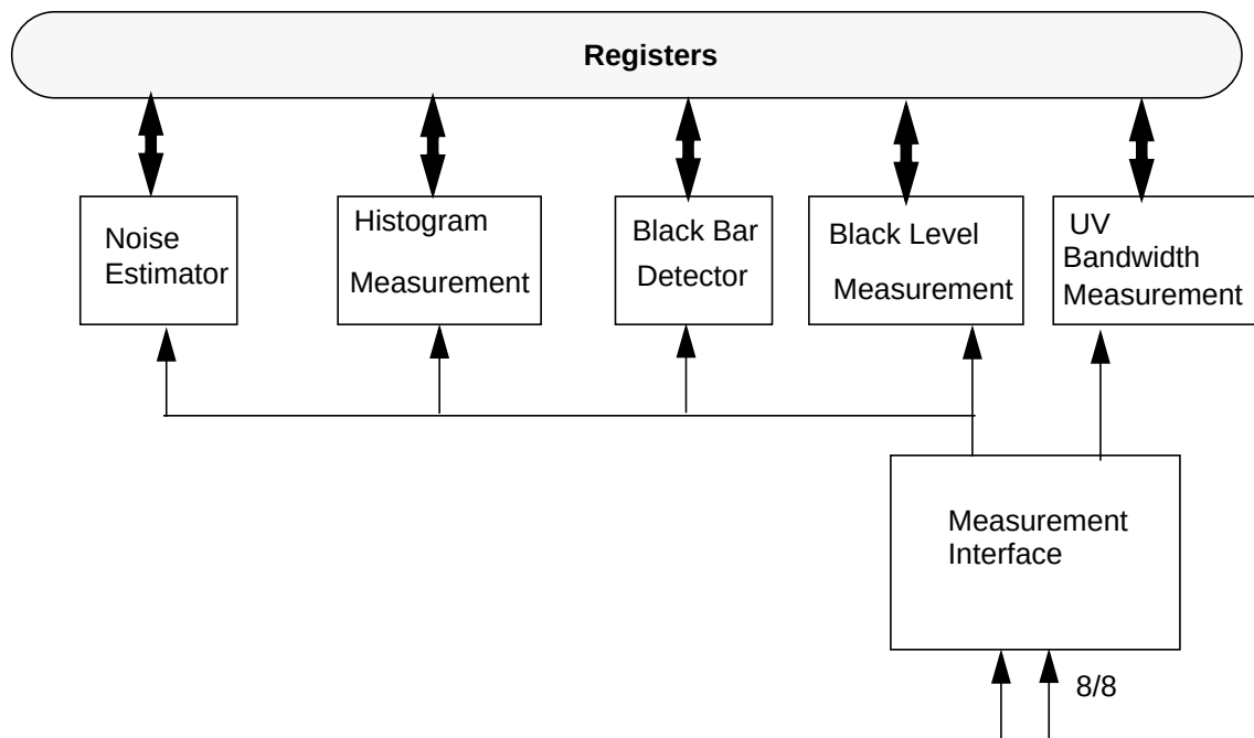
Figure 6: Measurement in the MBS
