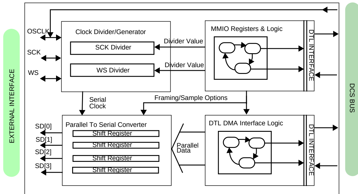
Figure 1: Audio Out Block Diagram
