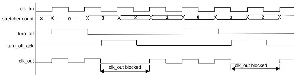
Figure 5: Clock Stretcher
