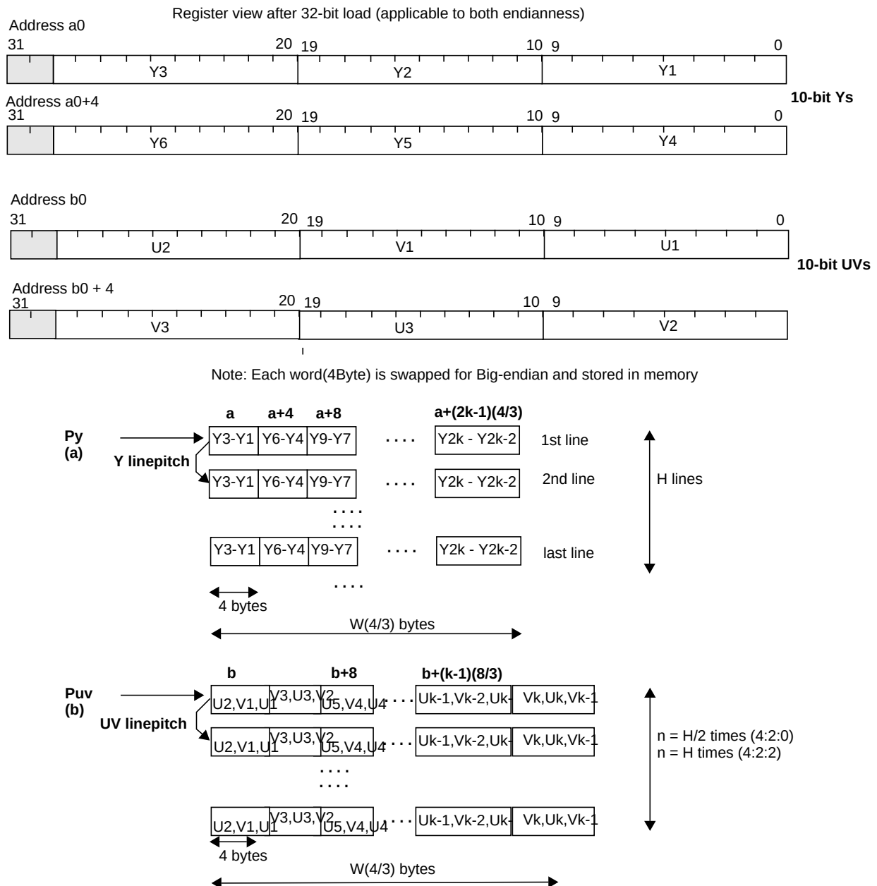
Figure 11: Semi-Planar 10-bit YUV 4:2:0 and YUV 4:2:2 Formats
