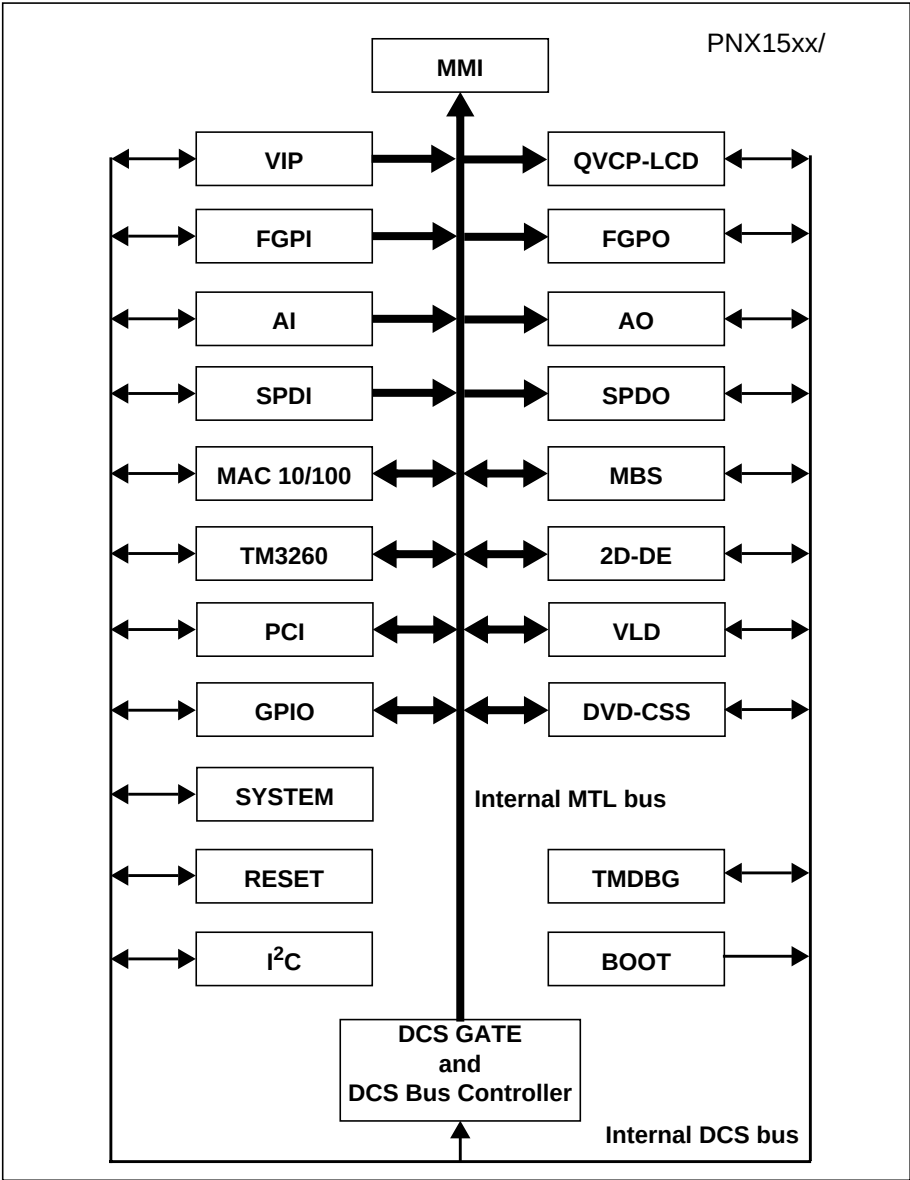
Figure 3: Simplified Internal Bus Infrastructure
