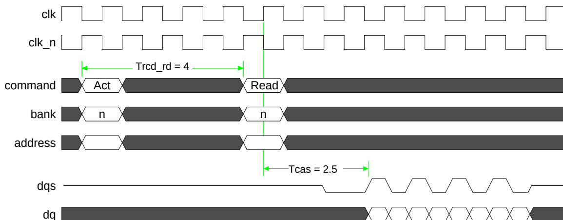
Figure 15: Trcd_rd Timing Parameter
