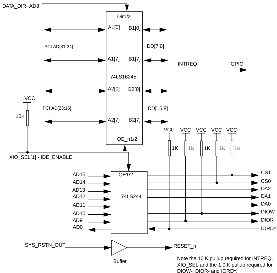
Figure 12: Isolation Translation Logic
