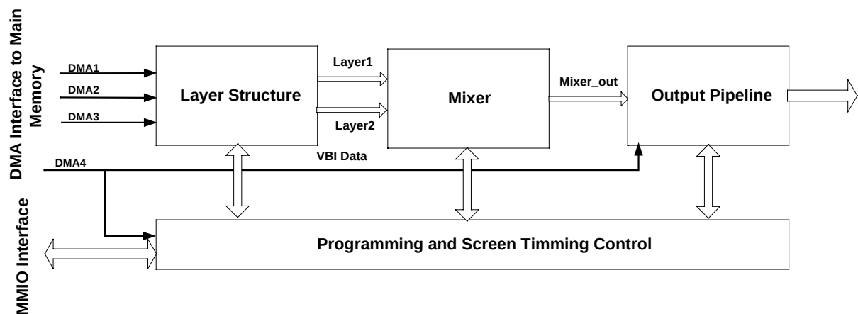
Figure 1: QVCP Top Level Diagram
