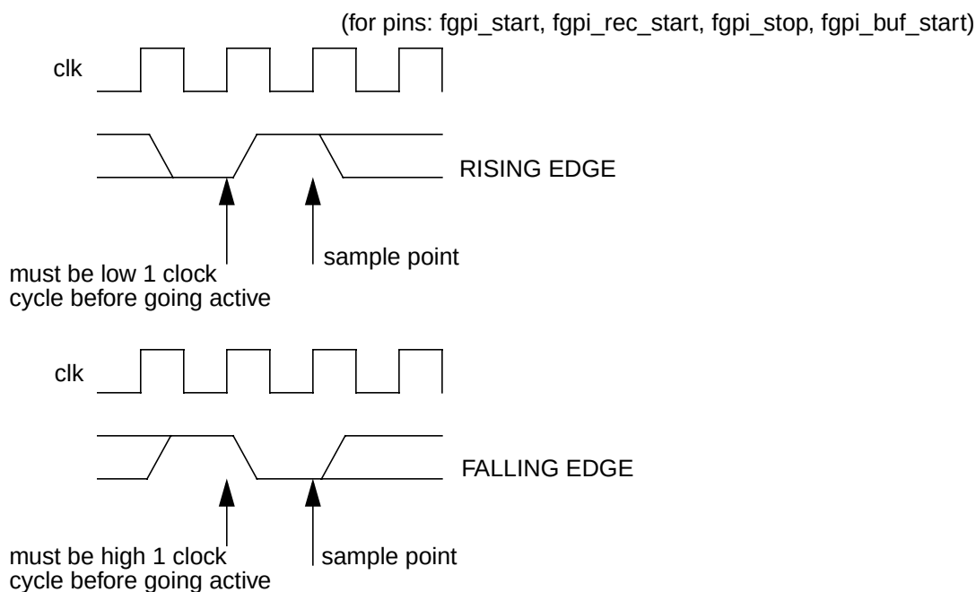
Figure 6: Signal Edge Definition
