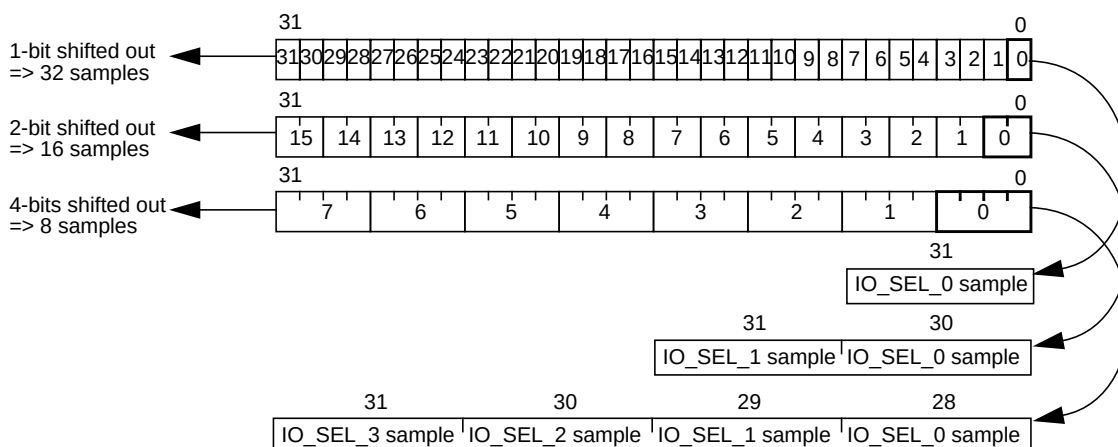
Figure 7: Up to 4-bit Samples per FIFO in Pattern Generation Mode
