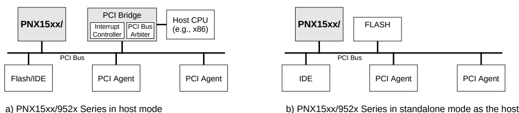
Figure 1: The Two Operating Modes of PNX15xx/952x Series
