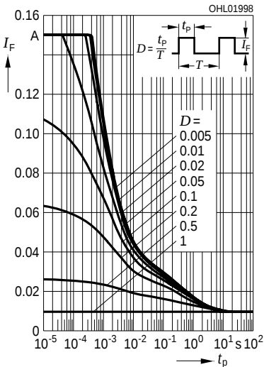
Zulässige Impulsbelastbarkeit I_F = f(t_p) Permissible Pulse Handling Capability LT; Duty cycle D = parameter, T_A = 85\text{ °C}
