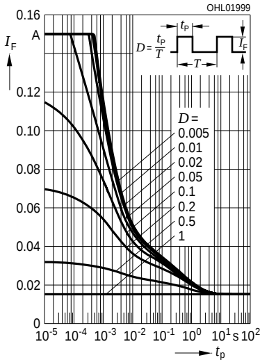
Zulässige Impulsbelastbarkeit I_F = f(t_p) Permissible Pulse Handling Capability LT; Duty cycle D = parameter, T_A = 25\text{ °C}
