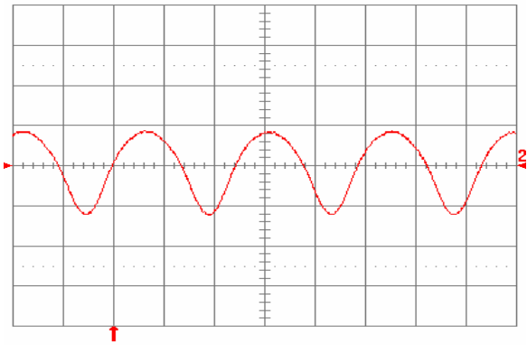
Fig. 1.2V.13: Input reflected ripple current, i_c (100 mA/div), measured at input terminals at full rated load current and V_{in} = 48 V. Refer to Fig. 1.2V.11 for test setup. Time scale: 1 µs/div.
