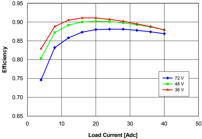
Fig. 2.0V.3: Efficiency vs. load current and input voltage for converter mounted vertically with air flowing from pin 3 to pin 1 at a rate of 300 LFM (1.5 m/s) and T_a = 25^\circ\text{C} .
