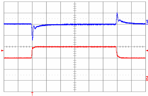
Fig. 1.0V.9: Output voltage response to load current step-change (20 A – 30 A – 20 A) at V_{in} = 48 V. Top trace: output voltage (100 mV/div.). Bottom trace: load current (10 A/div). Current slew rate: 1 A/ \mu s. C_o = 470 \mu F tantalum + 1 \mu F ceramic. Time scale: 0.2 ms/div.
