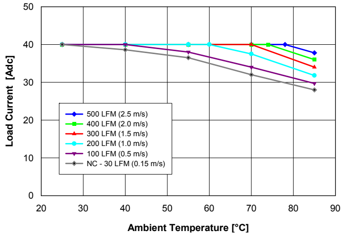
Fig. 1.0V.1: Available load current vs. ambient air temperature and airflow rates for QM48T40010 converter with B height pins mounted vertically with air flowing from pin 3 to pin 1, MOSFET temperature \leq 120^\circ\text{C} , V_{in} = 48\text{ V} .
