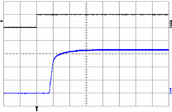
Fig. 3.3V.7: Turn-on transient at full rated load current (resistive) with no output capacitor at V_{in} = 48 V, triggered via ON/OFF pin. Top trace: ON/OFF signal (5 V/div.). Bottom trace: output voltage (1 V/div.). Time scale: 2 ms/div.
