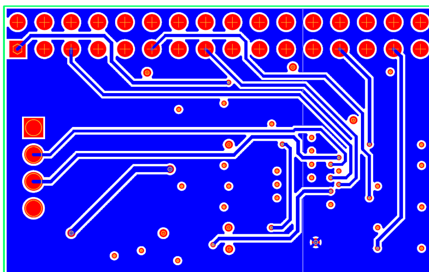
Figure 17 – Bottom layer
