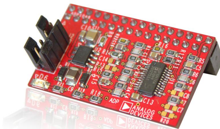
Figure 5 - ADP1047 daughter card
