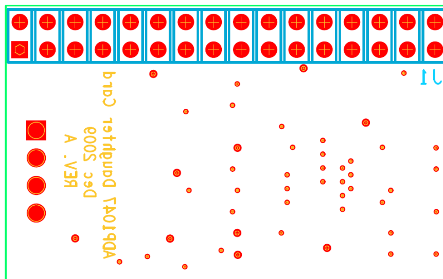
Figure 16 –Bottom Silkscreen
