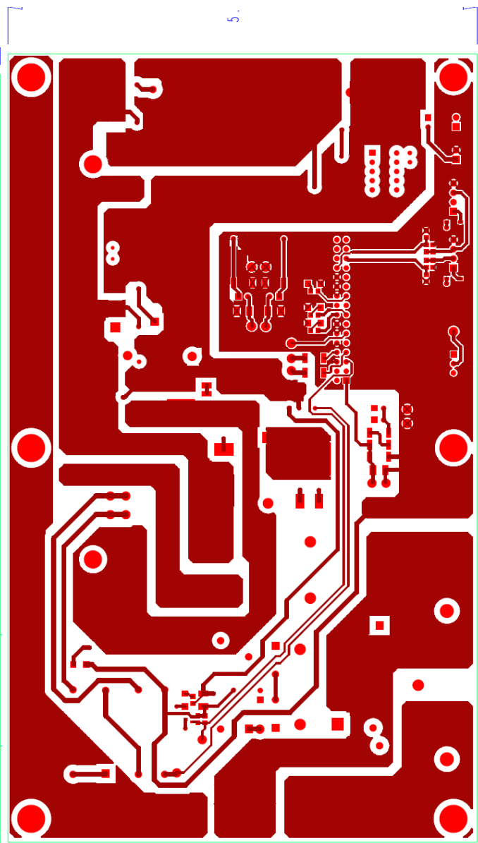
Figure 11 - Layout, Top layer
