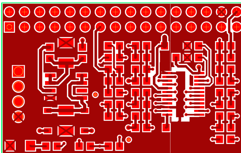
Figure 15 - Top Layer,
