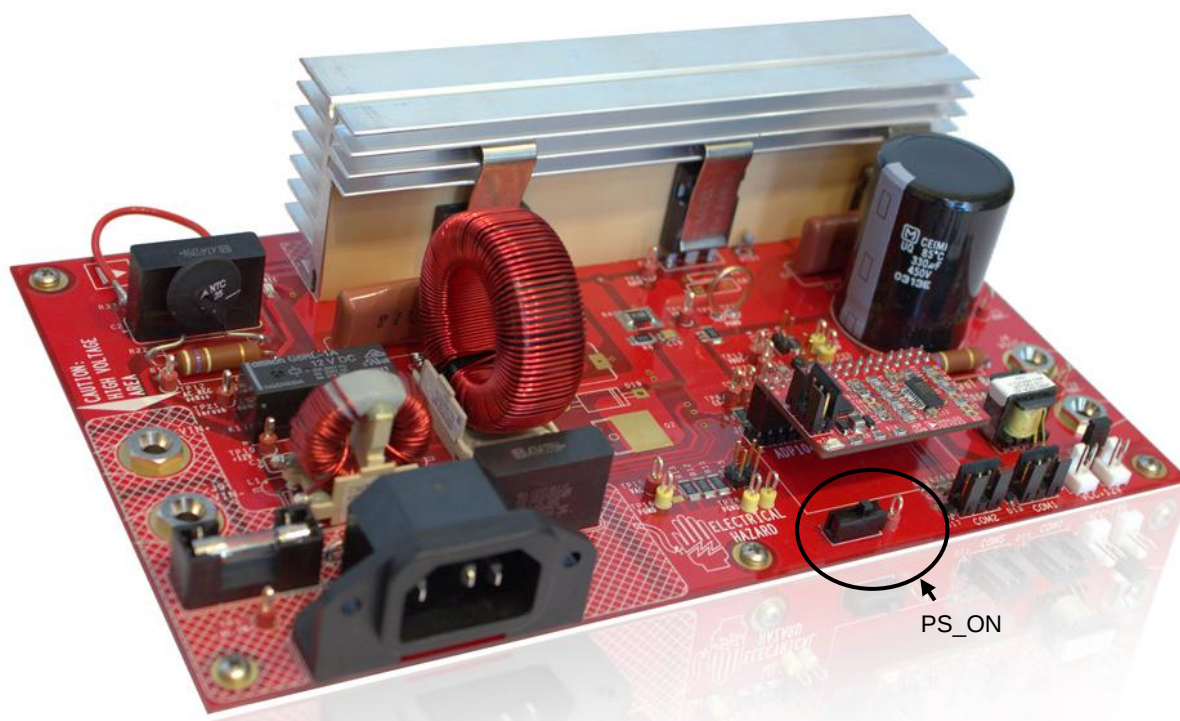
Figure 4 - 300W evaluation board showing PS_ON hardware switch
