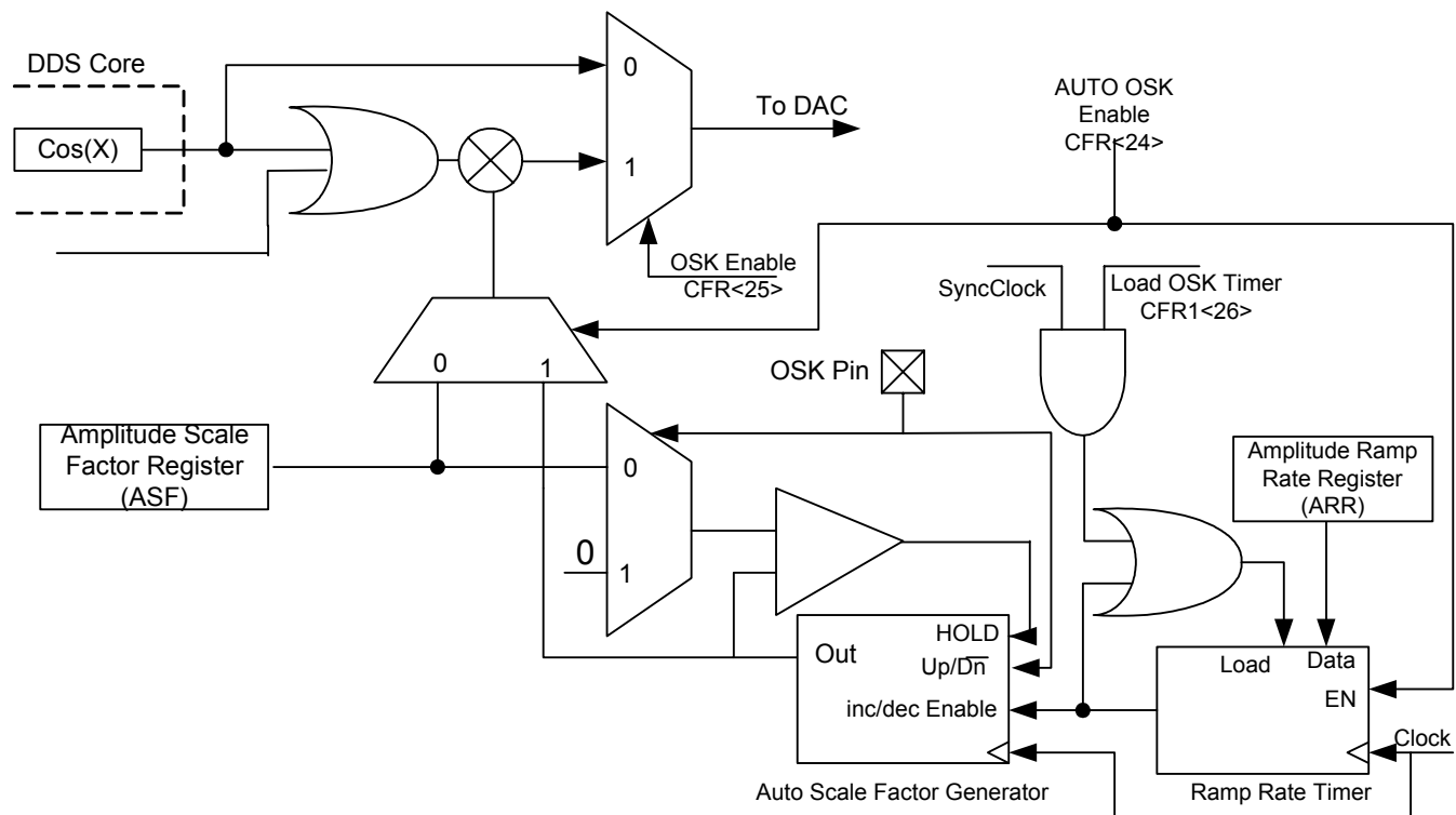
Figure C. On-Off Shaped Keying, Block Diagram
