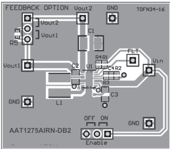
Figure 4: AAT1275A TDFN34-16 Package Evaluation Board Top Side Layout.
