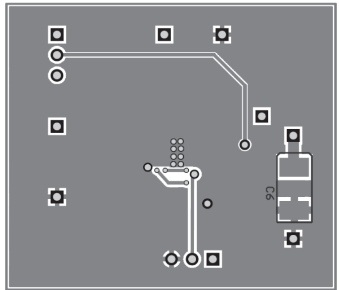
Figure 5: AAT1275A TDFN34-16 Package Evaluation Board Bottom Side Layout.
