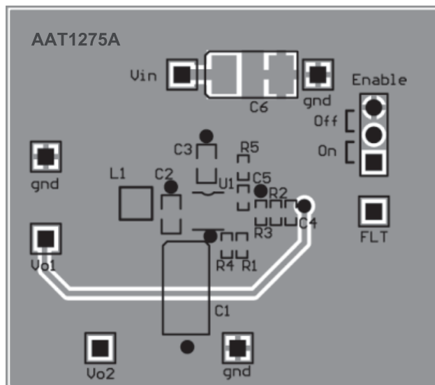
Figure 2: AAT1275A TSOPJW-12 Package Evaluation Board Bottom Side Layout.
