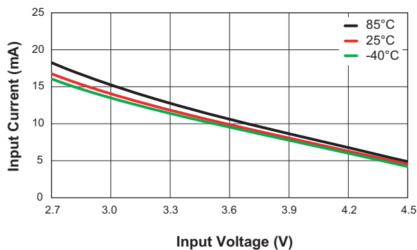
Quiescent Current vs. Input Voltage ( V_{OUT} = 5V ; No Load)
