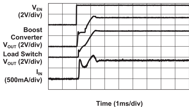
Enable Soft Start ( V_{IN} = 3.6V ; V_{OUT} = 5V ; I_{OUT} = 500mA )
