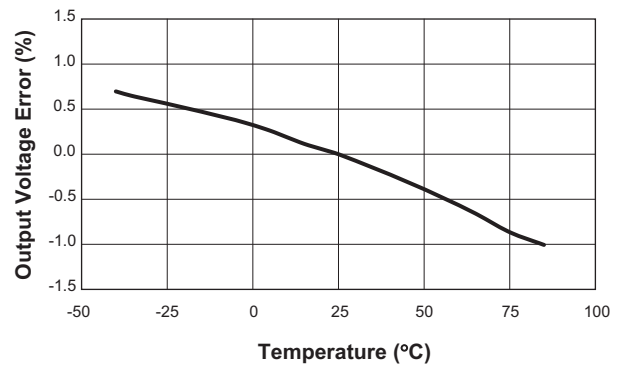
Output Voltage vs. Temperature ( V_{IN} = 3.6V ; V_{OUT} = 5V ; I_{OUT} = 100mA )
