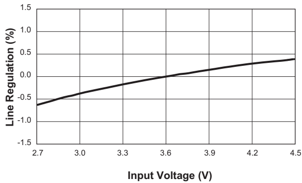
Line Regulation ( V_{OUT} = 5V ; I_{OUT} = 300mA )
