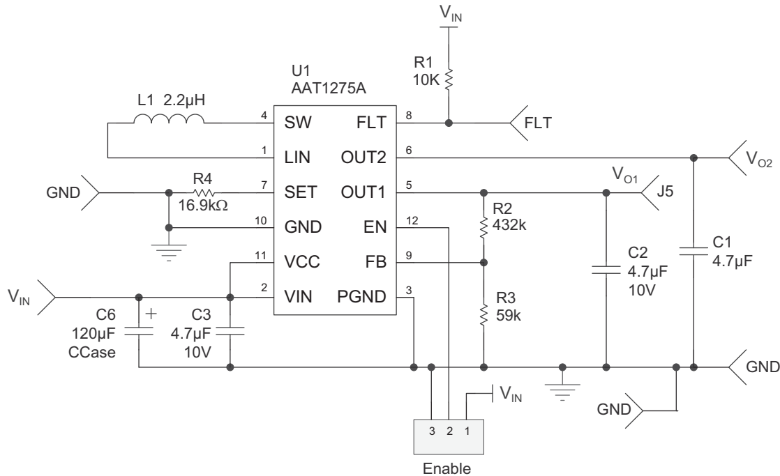
Figure 3: AAT1275A TSOPJW-12 Package Evaluation Board Schematic.
