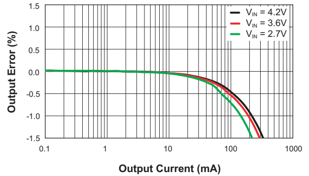
Load Regulation ( V_{OUT} = 5.0V )
