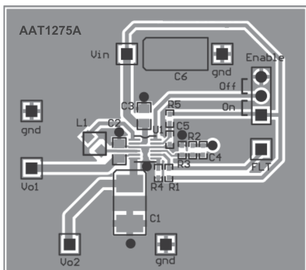
Figure 1: AAT1275A TSOPJW-12 Package Evaluation Board Top Side Layout.
