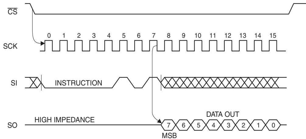
Figure 4-4. RDSR Timing
