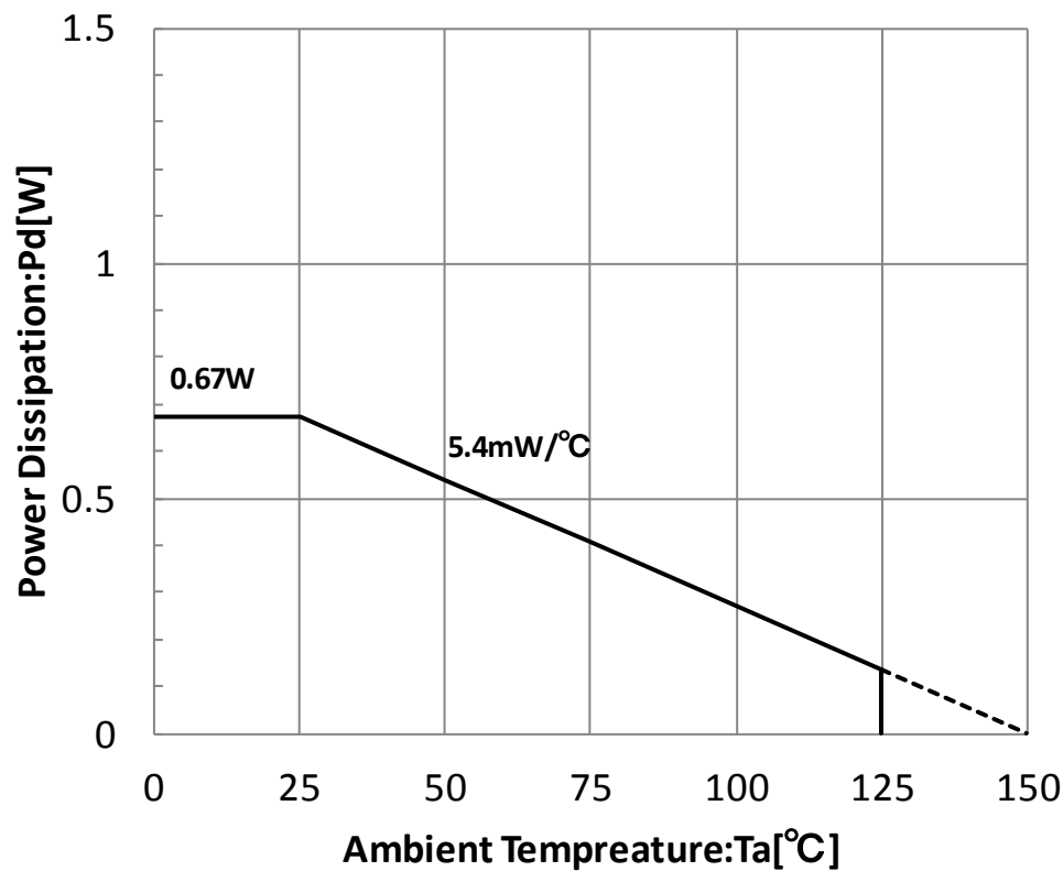
Figure 26. Power Dissipation(70mm × 70mm × 1.6mm t 4layer PCB)
