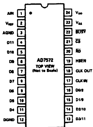
DIP
