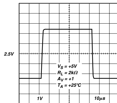
Figure 24. Large Signal Transient Response
