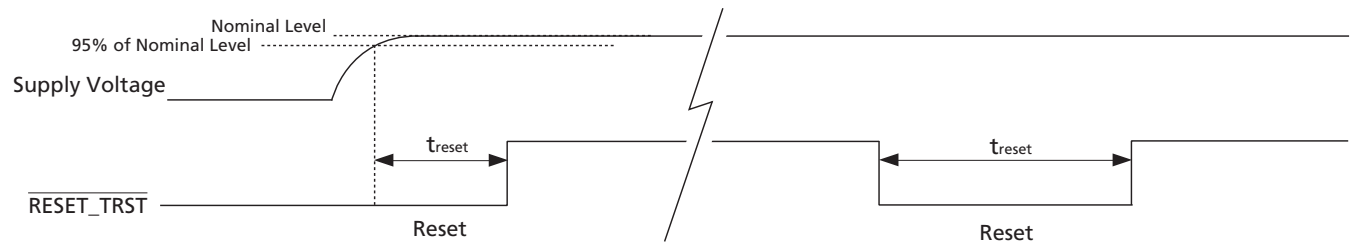
Figure 4-34: Reset Pulse
