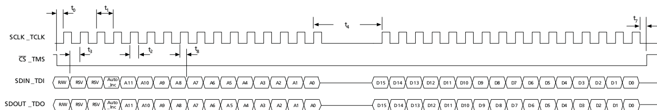
Figure 4-29:Write Mode
