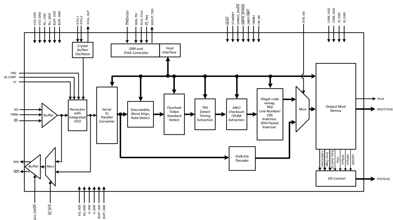
GS1660A Functional Block Diagram
